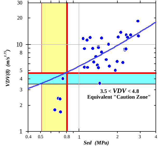
Figure 7. Cross-plot of VDV(8) against S_{ed} , showing the VDV(8) of 84% of repeated shocks signatures exceed a level of 4.8 m/s^{1.75} ( S_{ed} = 0.8 MPa).
