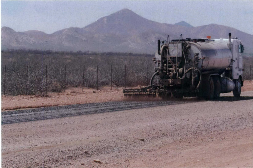
Photo 35. Application of asphalt emulsion by heated tanker with distribution bar
