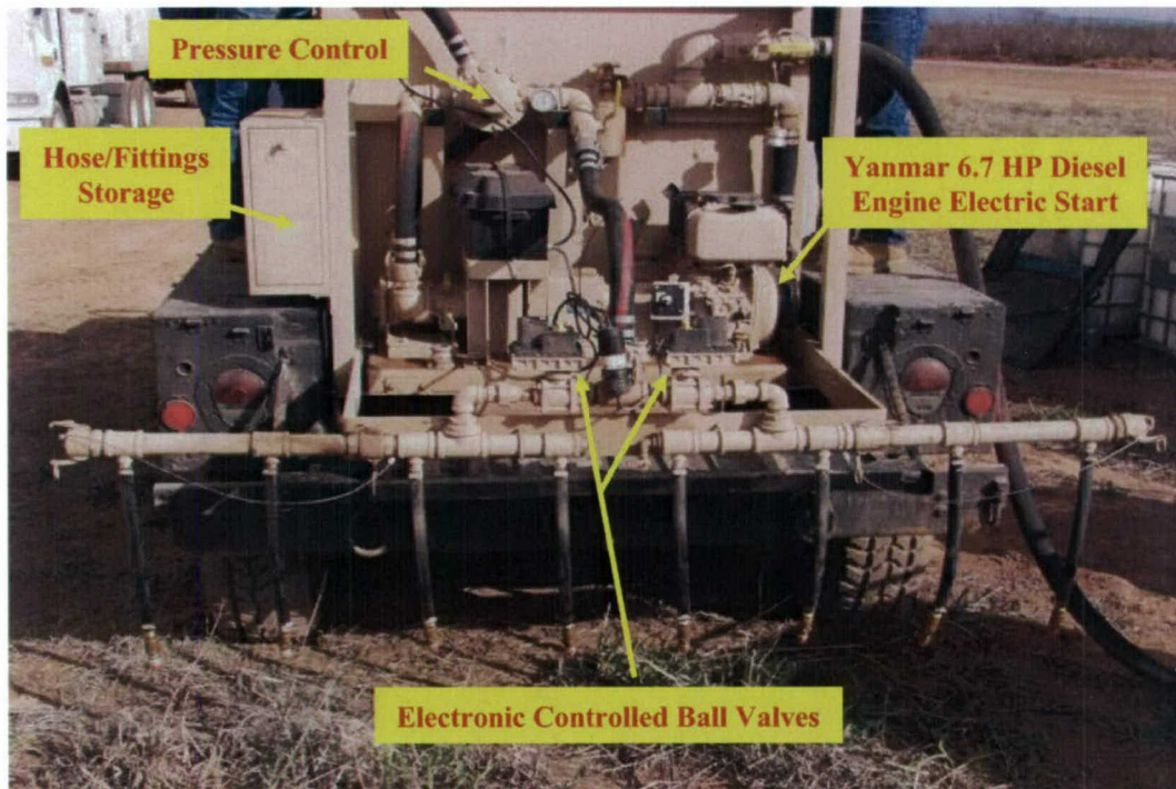
Photo 31. Basic components of spray unit
