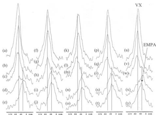
Figure 2. Selected 31 P NMR spectra obtained for VX added to concrete coupons at (top to bottom) 1 h, 5 h, 29 h, 4 days and 11days: one-4 \mu L drop (a-e); two-2 \mu L drops (f-j); four-1 \mu L drops (k-o), eight-0.5 \mu L drops (p-t) and twenty-0.2 \mu L drops (u-y).
