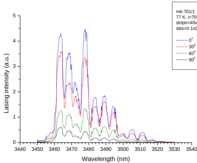
Fig.1.10. Polarization features of lasing spectra for the hybrid InAsSbP/InAsSb/CdMgSe laser structure
