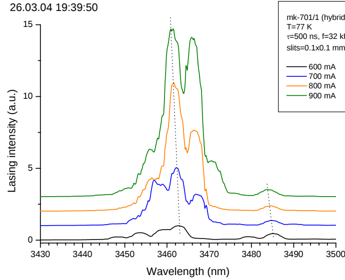
Fig.1.9. Blue shift of mode picture for the hybrid InAsSbP/InAsSb/CdMgSe laser structure with drive current increasing above the threshold
