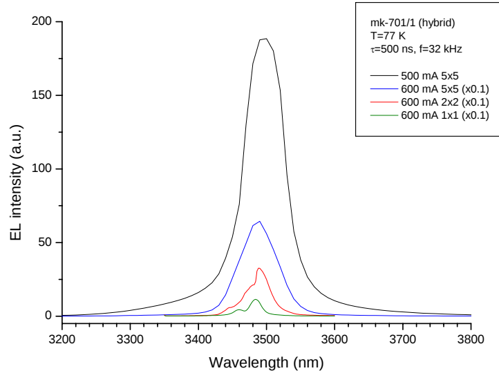
Fig.1.7. EL spectra for the hybrid InAsSbP/InAsSb/CdMgSe laser structure near the lasing threshold for various slits width.
