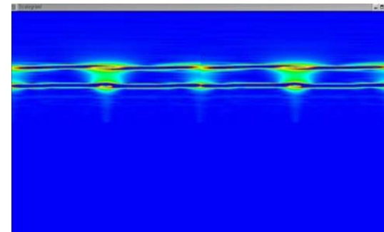
CWT Scalogram
