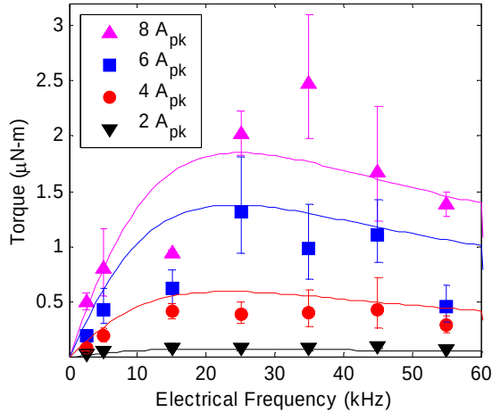
Fig. 9. Torque vs. electrical frequency for NiFe induction machine at 50 \mu\text{m} air gap. Measurements at different peak currents are indicated with points, and theory with solid curves.
