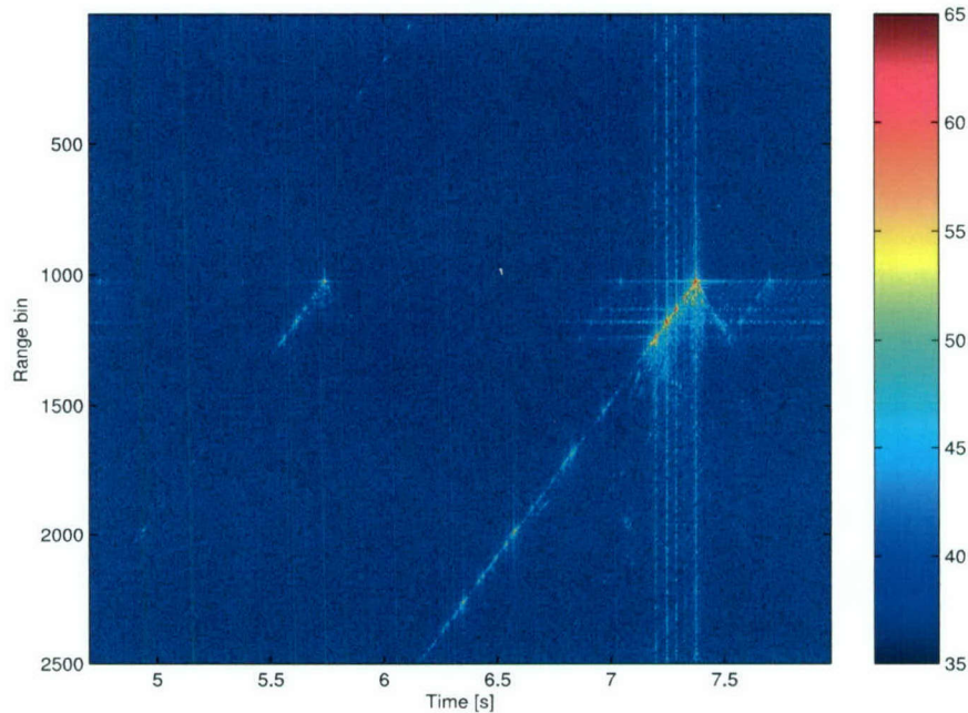
Figure 22 : Range and Doppler compressed bistatic SAR data.
