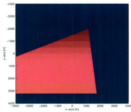
(e) Bistatic angle = 150^\circ .
