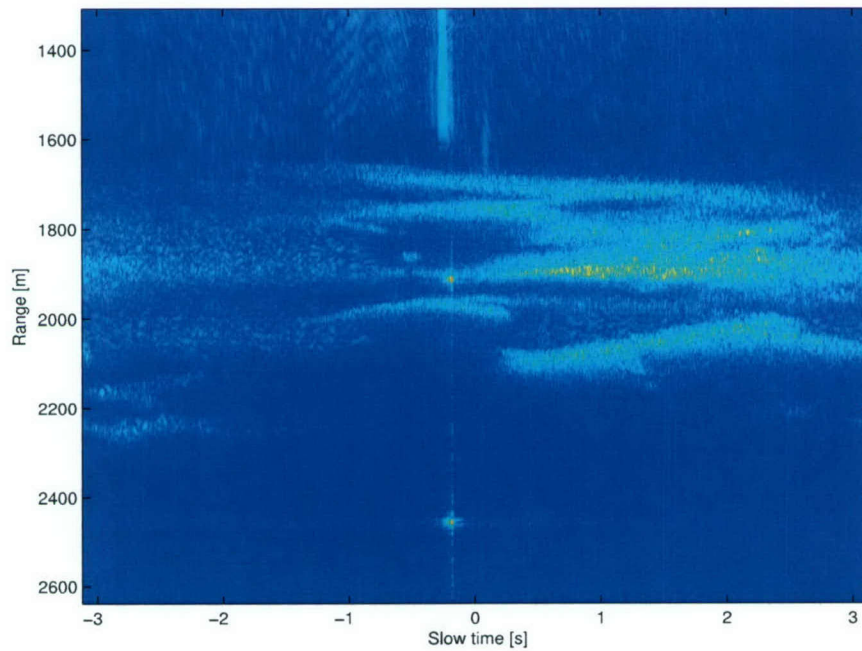
Figure 31 : Bistatic SAR image for the 1 Nov. 2002 airborne trial around ARC location.
