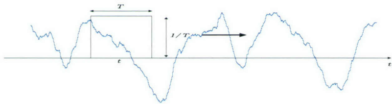
Figure B.1 : Realisation of phase noise with sliding window to estimate the rms for finite observation time T .
