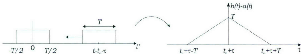
Figure 3 : Illustration of integration interval for range-compression.
