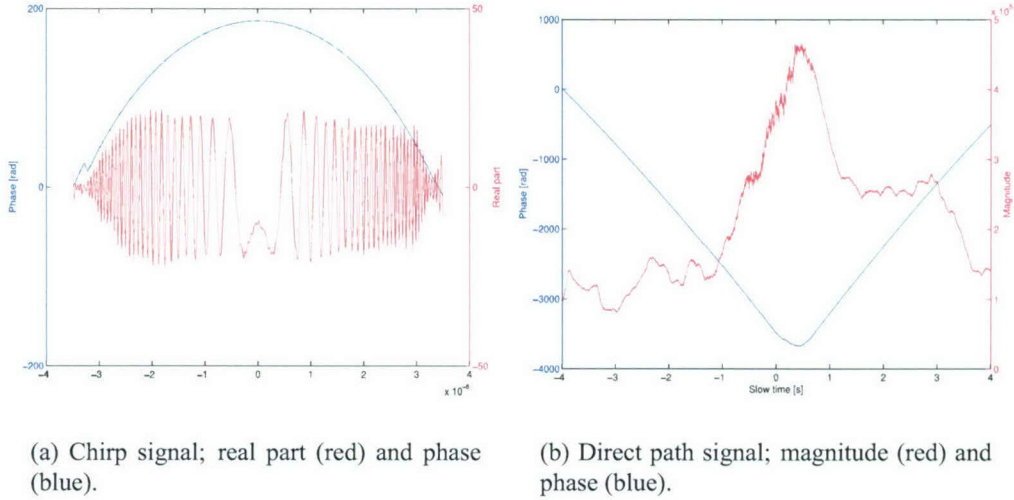
Figure 26: Received chirp and direct path signals (magnitude and phase).
