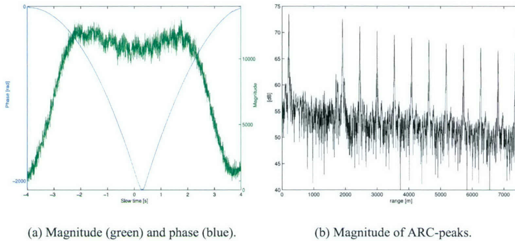
Figure 27: Magnitude and phase of ARC-signal at 3 km range and magnitudes of ARC-peaks along range.
