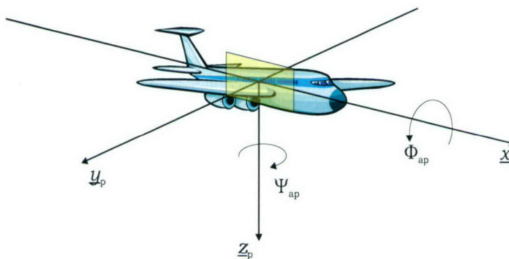
Figure E.3 : Angular relation between platform and antenna coordinate systems.
