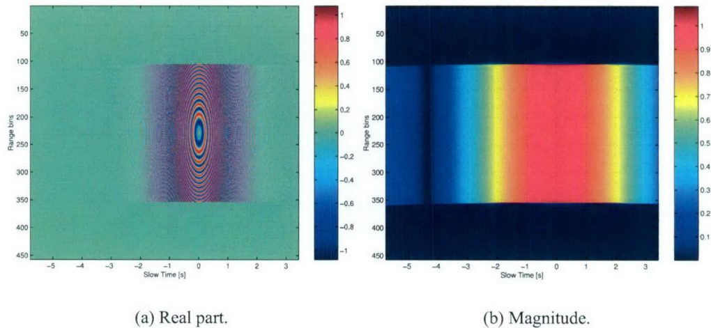
Figure 15: Real part and magnitude of simulated bistatic raw data for an airborne transmitter and stationary receiver configuration, \Psi_{0,2} = 90^\circ .
