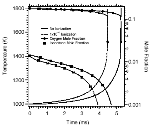
Figure 6. Species concentration and temperature as a function of time for 1.4% C_8H_{18} , 17.6% O_2 , 1% NO , 80% Ar combustion ( I_t=1 ) at a constant pressure of 1 atm, T_{initial}=1000 K with (dashed lines) and without (solid lines) ionization.
