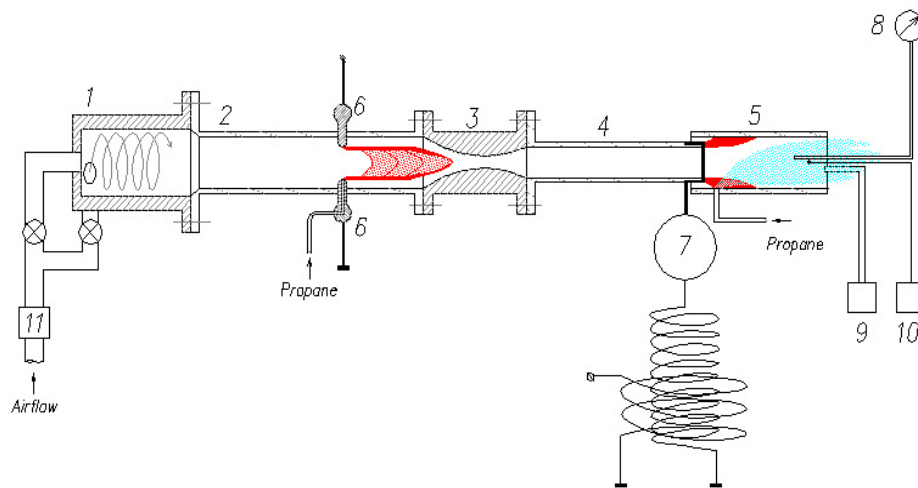
Fig.2.1. 1, 2- fore-chamber with electric arc pre-heater, 3- nozzle, 4, 5- test section, 6-arc electrodes, 7- HF electrode, 8- pressure sensor, 9-chemical probe, 10- thermocouple, 11- mass airflow
