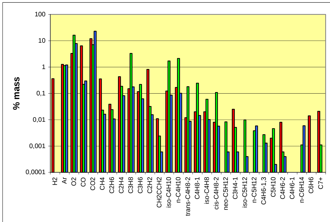
Fig.1.2. PAC species in the HWT-1 without separation zone. Green - a lean propane-butane mixture in subsonic airflow \phi < 2 ; red - rich propane-butane mixture, \phi < 0,125 ; blue - \phi \approx 1
