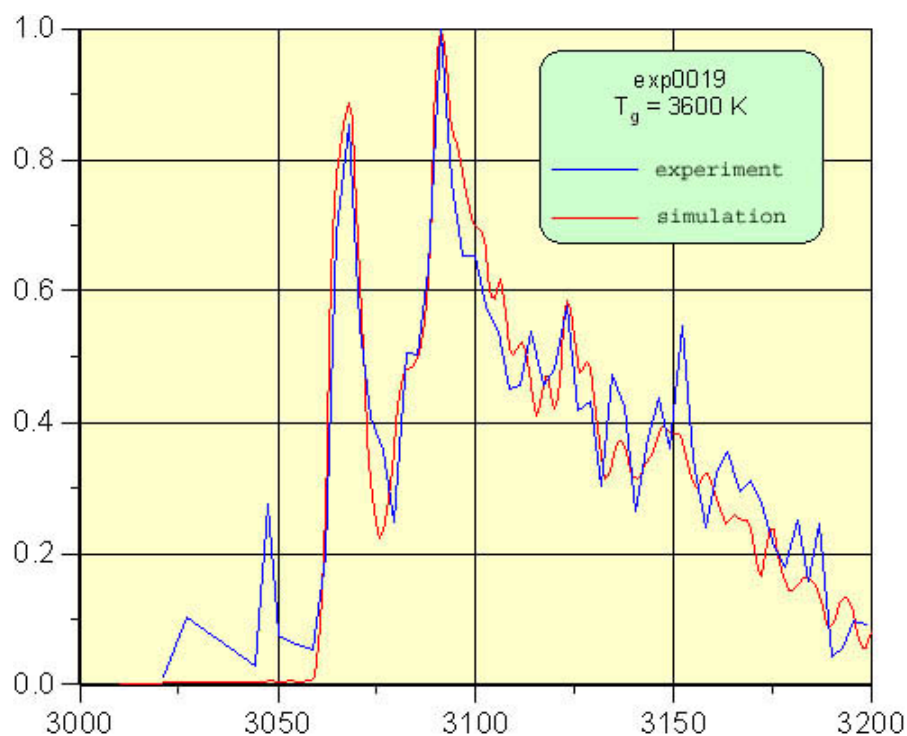
Fig.1.13. Optical spectrum of the OH radical. Blue – experiment, red – simulation. Pre-heater on , electric power N_e=425\text{W} , airflow velocity 10 m/s, static pressure P_{st}=1\text{ Bar} , \Phi=1,81 , static temperature T=415\text{C} , gas flow temperature behind PAC zone - T_f=930\text{C}
