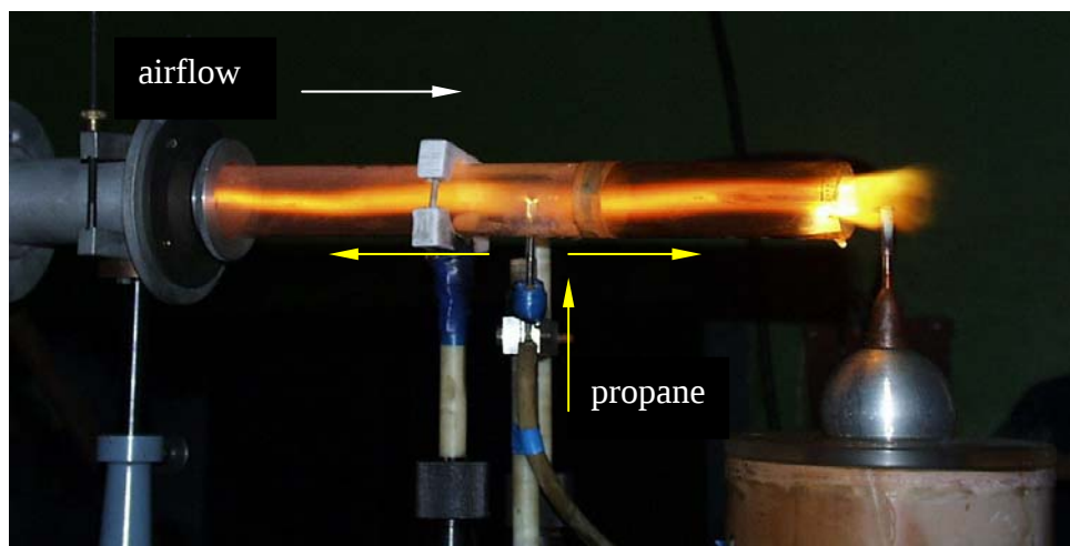
Fig.2.5. Propane transportation through HF filament discharge. Red colour is typical chemical flame colour in high-speed airflow in this regime ( \text{CH}_2 generation), M=1,2 , P_{st}=1 Bar, \phi=0,7
