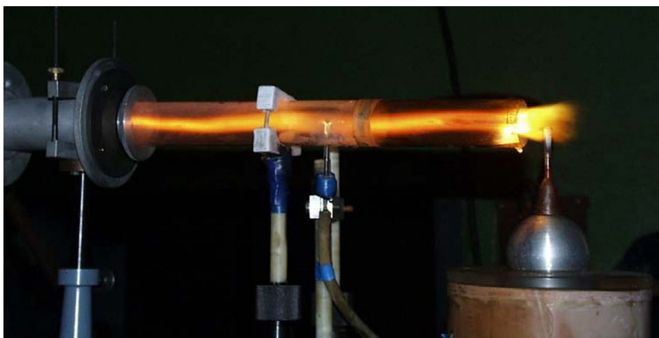
Fig.1.14. Internal PAC. Red flame. HF discharge. M=1,2 ; P_{st} \sim 1 Bar, fuel-airflow equivalence ratio \phi=0,7 ; CH_2 radical generation
