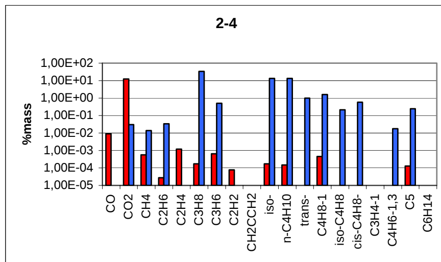
Fig.2.6. Chromatographic analysis of final PAC species, (log scale). Combined electric discharge (DC+ high voltage pulses), M=0,3 ; P_{st}=1 Bar, \phi \sim 1,5 . Blue – initial airflow-fuel mixture, red- PAC
