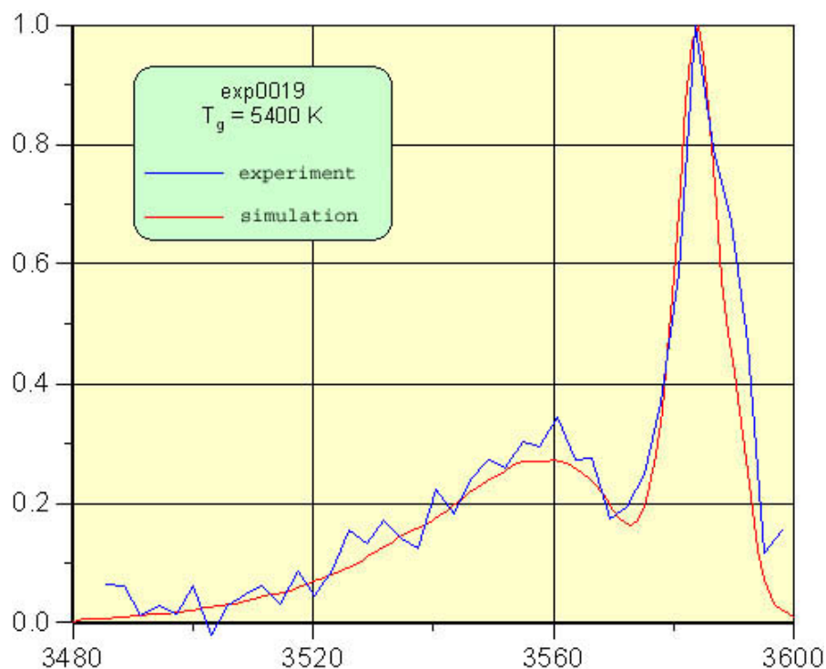
Fig.1.12. Optical spectrum of the CN(1,0) radical. Blue – experiment, red – simulation. Pre-heater on , electric power N_e=425\text{W} , airflow velocity 10 m/s, static pressure P_{st}=1\text{ Bar} , \Phi=1,81 ; static temperature T=415\text{C} , gas flow temperature behind PAC zone - T_f=930\text{C}
