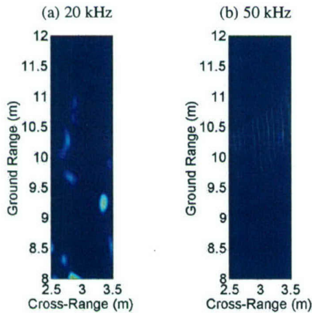
Fig. 5. SAS images for a flattened bottom.
