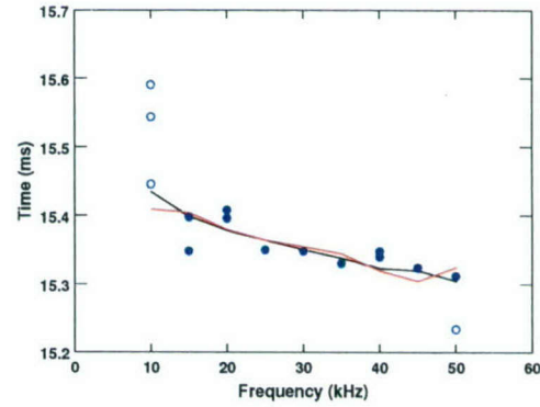
Fig. 6. Two-way time versus frequency.
