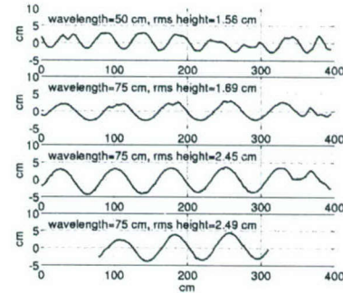
Fig. 3. Measured ripple profiles.
