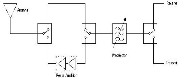
Fig. 1: Generic wideband SDR RFFE
