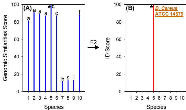
Fig. 7. Percentages of accepted peptides from the analysis of a B. cereus ATCC 14579 protein digest matched to proteomes of database bacteria from the family Bacillaceae (A). (B) the corresponding identification plot obtained by filtering out the degenerate sequences found in (A). Abbreviations: a, B. anthracis strains (species 1-4); c, B. cereus strains (5,6), h, B. halodurans (7); s, B. subtilis (8); i, Oceanobacillus ihyensensis (9); t, B. thuringiensis (10). For the number assigned to a particular strain – see Fig. 9.
