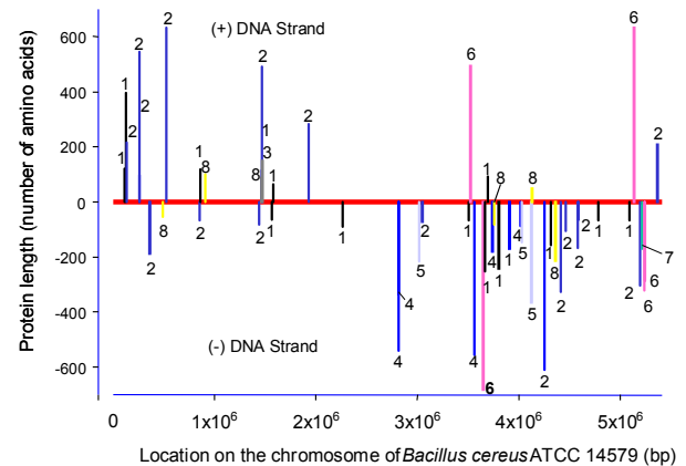
Fig. 8. Locations of genes encoding proteins that contributed peptides identified during LC-MS/MS analysis of a protein extract from B. cereus ATCC 14579 on its circular chromosome. Vertical axis indicates sizes of these proteins expressed as a number of amino acids. Functional categories of proteins: 1-information processing; 2-cellular processing; 3-coenzyme and cofactor metabolism; 4-membrane transport; 5-amino acid metabolism; 6-energy metabolism; 7-nucleotide metabolism; 8-hypothetical.
