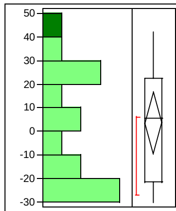
Figure 13. Cargo Prediction Errors
