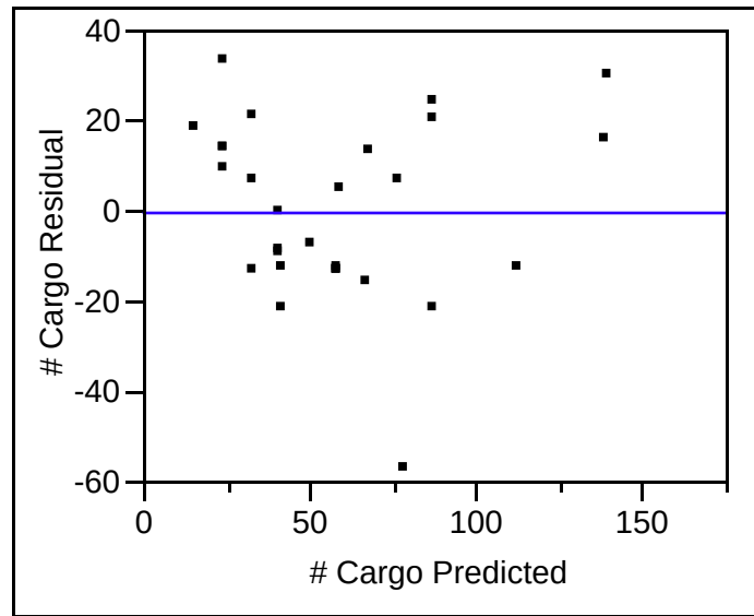
Figure 12. Residual for Predicted Plot for Cargo Model
