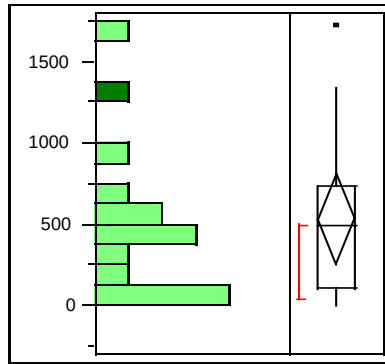
Figure 14. Squared Cargo Prediction Errors
