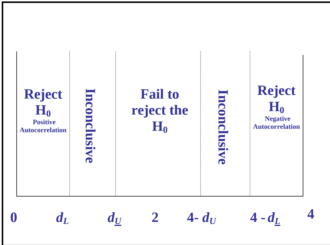
Figure 8. Durbin-Watson Critical Value Range
