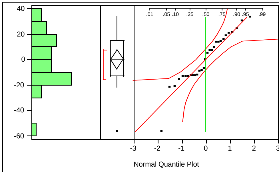
Figure 11. Normal Quantile Plot of Cargo Model Residuals
