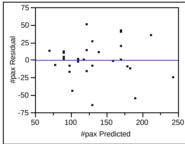
Figure 10. Residual by Predicted Plot for Passenger Model
