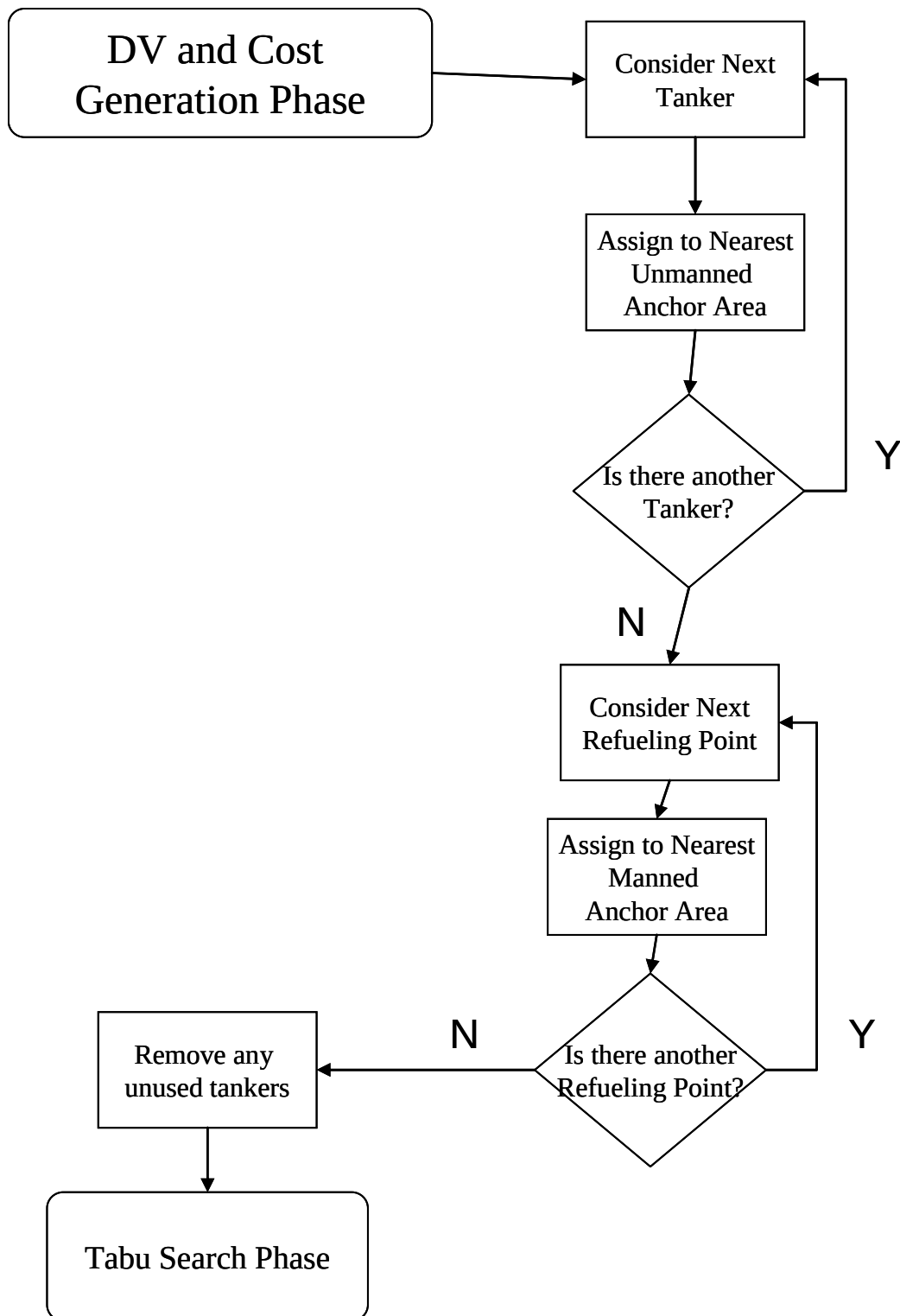
Figure 7: Initial Solution Generation Phase
