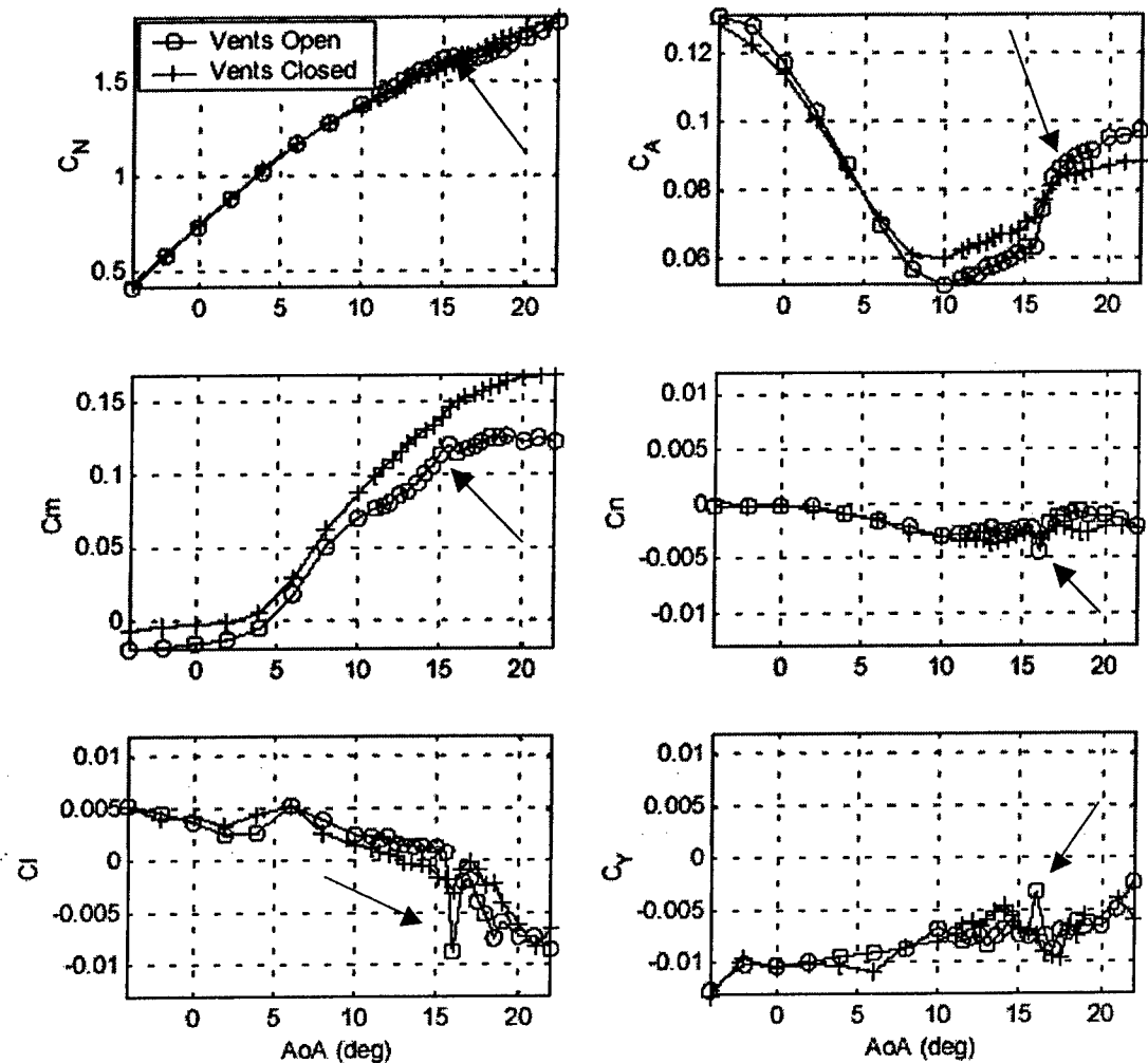
Figure 1-4: Results from Cook [3], "Effect of LEX vent deflection on F/A-18E configuration, LEF=10°, TEF=30°, and AIL=30°"
