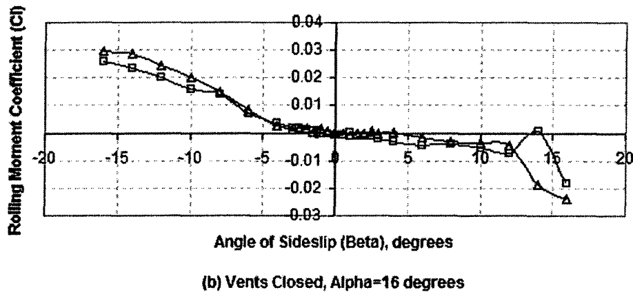
Figure 3-2 (a, b): Effect of Vertical Tail at Angle of Attack 16^\circ
