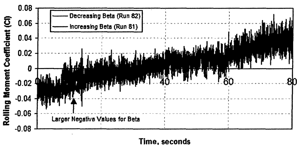
Figure 3-8: Rolling Moment Coefficient Hysteresis Analysis at 16.5° Angle of Attack, Static Data
