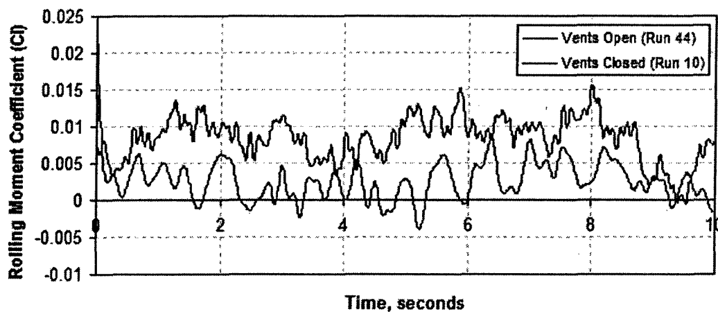
Figure 3-21: Rolling Moment Coefficient Time History
