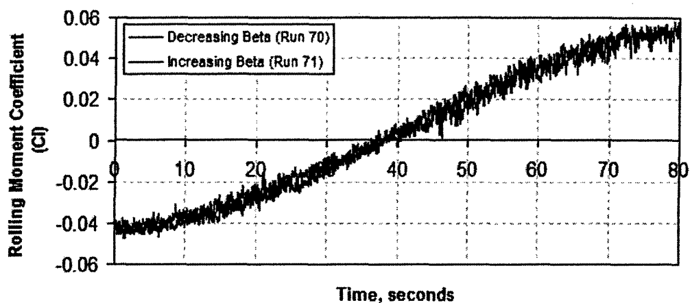
Figure 3-7: Rolling Moment Coefficient Hysteresis Analysis at 10° Angle of Attack, Static Data
