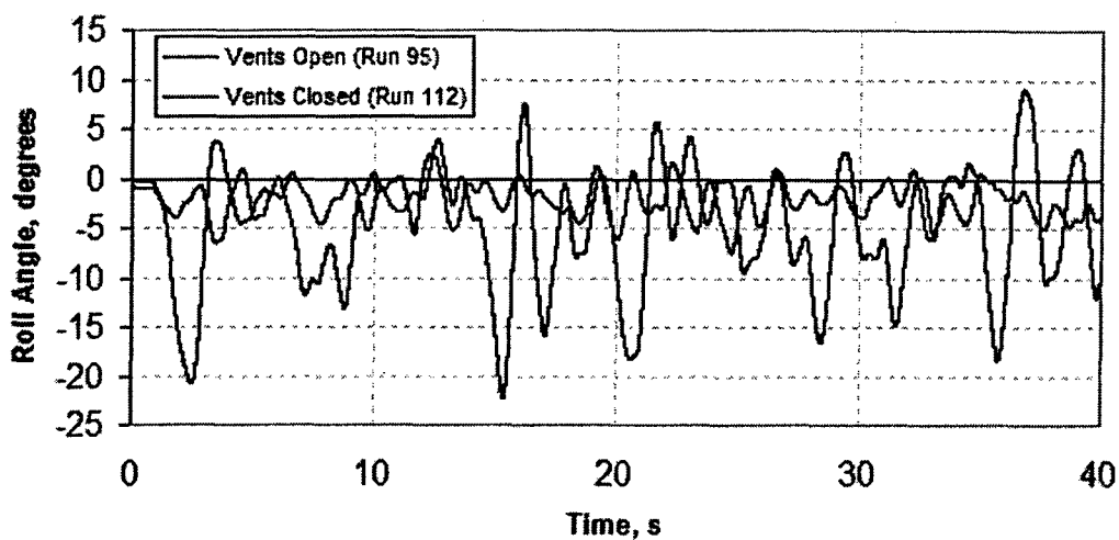
Figure 3-12: Lateral Motion Analysis for Vents Open and Vents Closed, Angle of Attack 13°, FTR
