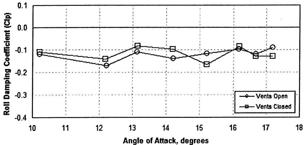
Figure 3-10: Roll Damping Effects [2], FTR Data
