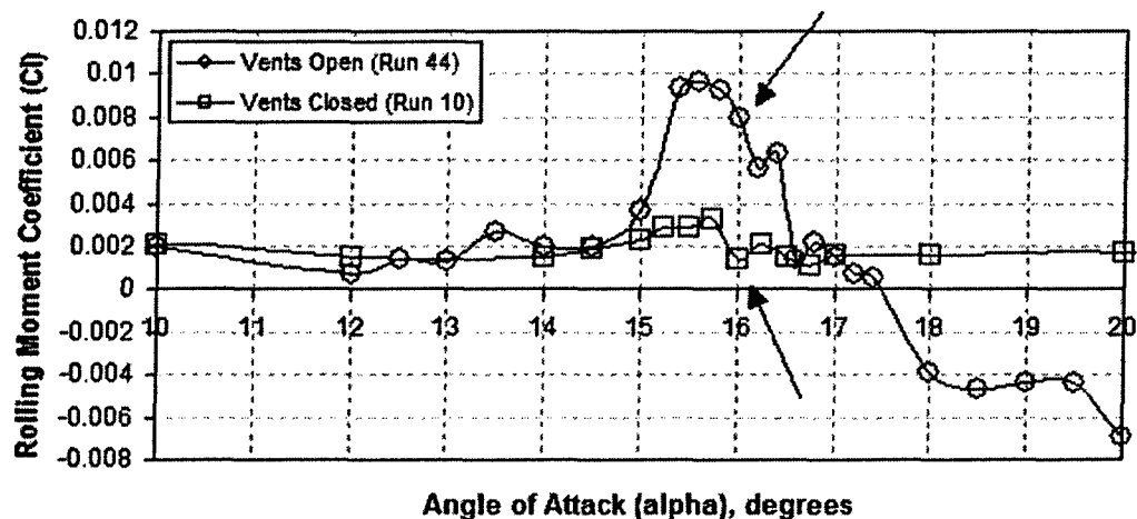
Figure 3-13: Time-Averaged Static Rolling Moment Coefficient, Static Data
