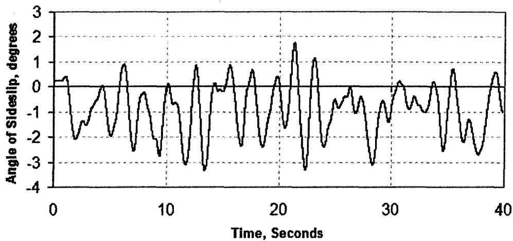
Figure 3-19: Angle of Sideslip Time History for Angle of Attack 15°, FTR Data.
