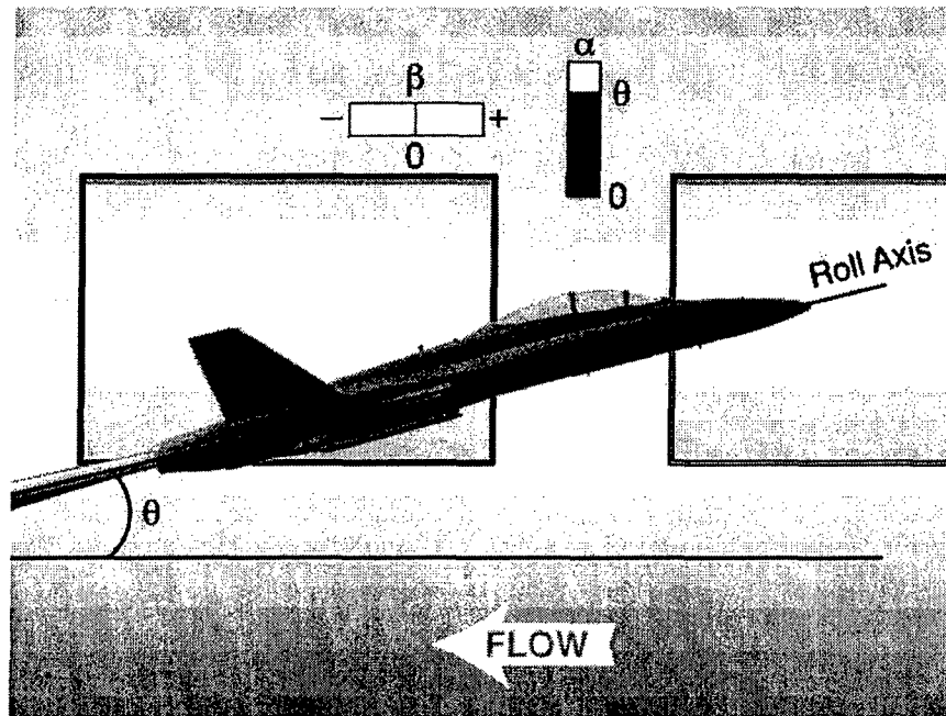
Figure 2-5: Kinematics of FTR Setup
