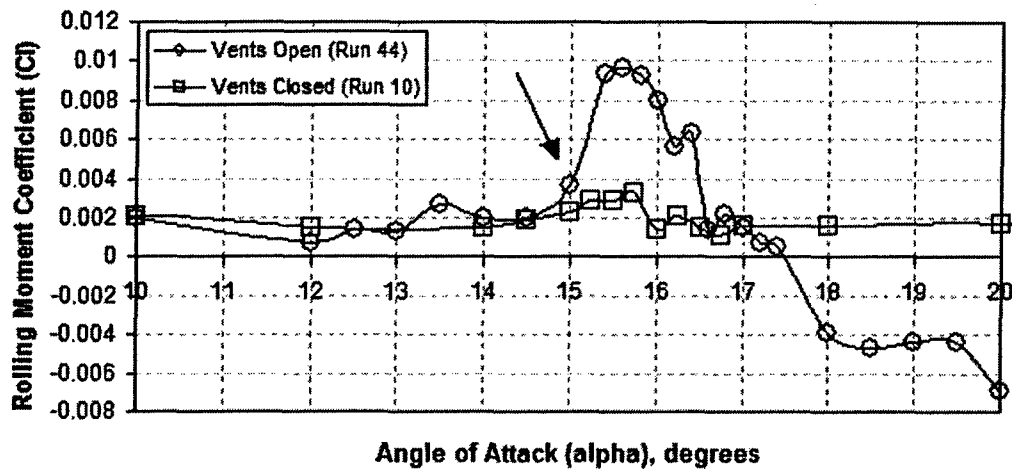
Figure 3-13: Time-averaged Static Rolling Moment, Static Data
