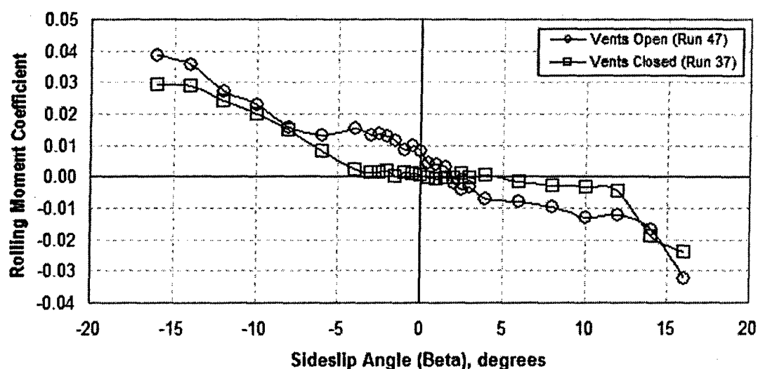
Figure 3-22: Beta vs. Rolling Moment Coefficient for Angle of Attack 16°, Static Data
