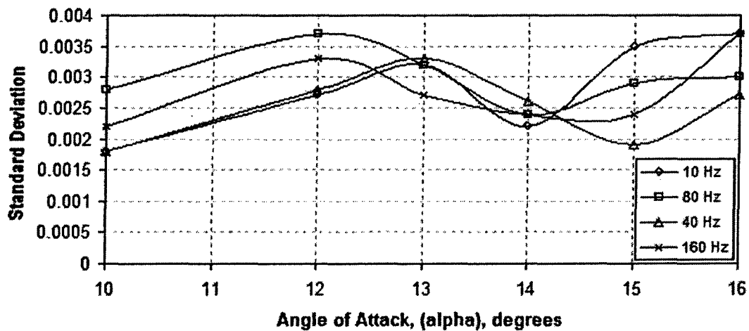
Figure 2-4: Standard Deviation Comparison, Static Data
