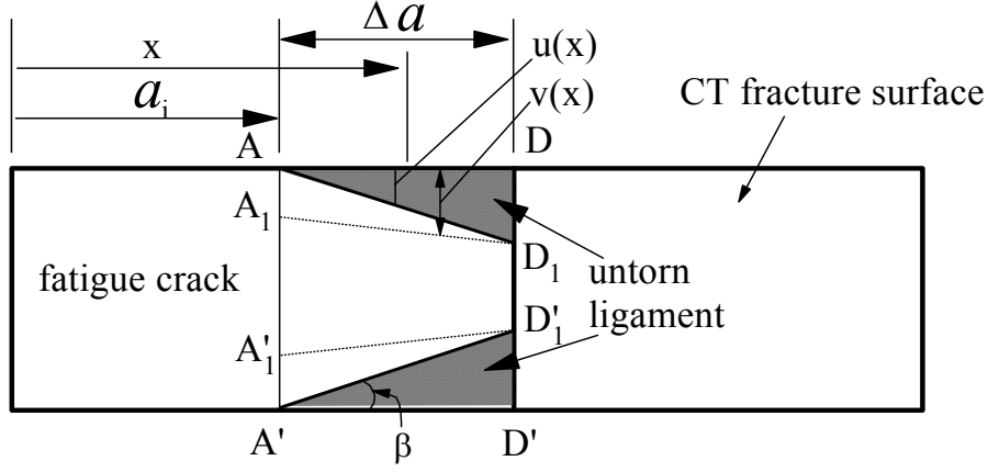
Fig.6-5 Schematic of Schijve's model
