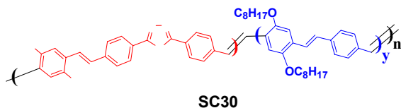
Figure 2. Structure of the statistical copolymer (SC30), which has on average 70% oxadiazole containing PPV monomer and 30% PPV monomer. Composition of the copolymer was deduced from NMR.
