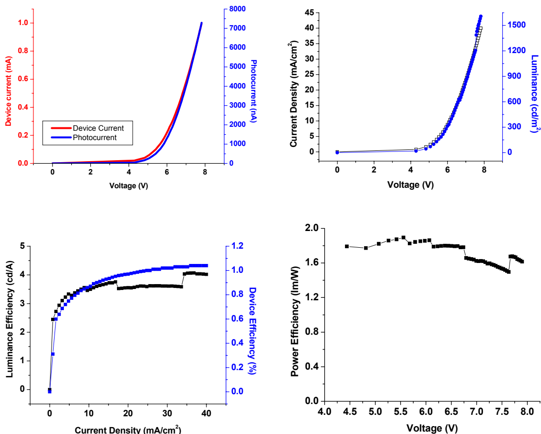
Figure 4. Characteristics of device made on plastic substrate with PEDOT/PSS , LiF and aluminum cathode (a) device current versus photocurrent, (b) brightness in \text{cd/m}^2 , (c) external quantum and luminance efficiencies and (d) power efficiency.
