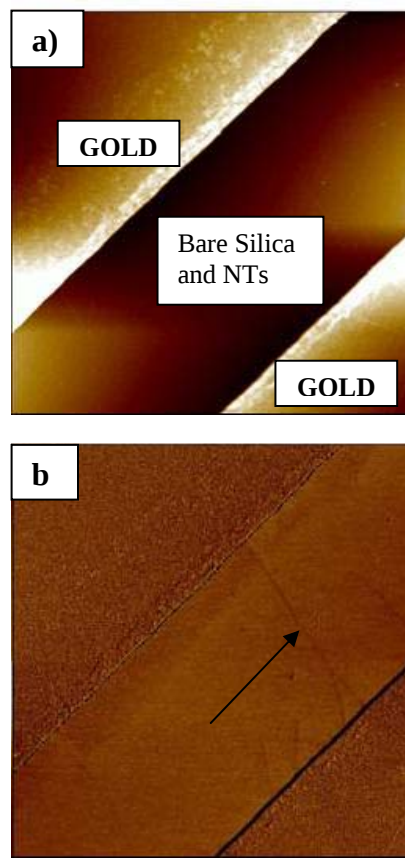
Figure 3. (a) 15x15 \mu\text{m}^2 AFM height image of two gold pads separated by a 7.2 \mu\text{m} gap. (b) AFM phase image of (a) where a SWNT is seen bridging between the two electrodes (indicated by arrow).
