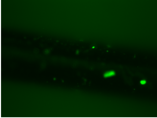
Figure 5. Fluorescence image of CdSe-ZnS/CdS/CdSe-ZnS/CdS-coated Au wire with a collection window of 525 \pm 20 nm.
