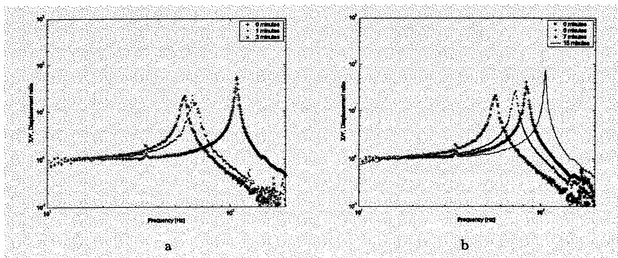
Figure 7: (a) Frequency response measurements during the softening of the polymer; (b) frequency response measurements during the stiffening of the polymer.
