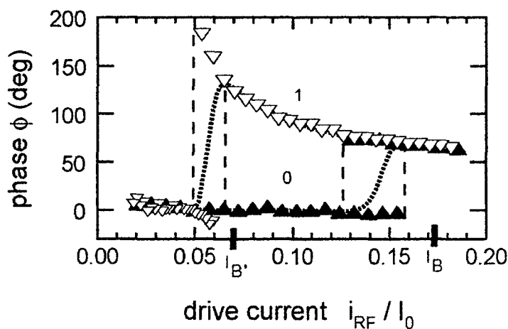
Figure 2: Reflected signal phase \phi as a function of drive current i_{RF}/I_0 . I_0=1.172\mu A ; (\omega_p-\omega)/\omega=0.122 . Symbols denote the mode of \phi with up and down triangles corresponding to increasing and decreasing current, respectively. The dotted line is \langle \phi \rangle . The calculated bifurcation points, I_{B'} and I_B , are marked on the horizontal axis. The 0 and 1 phase states are reminiscent of the superconducting and dissipative states of the DC current biased junction.
