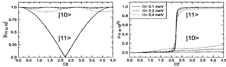
Figure 2: Amplitude (left) and phase (right) of states |10\rangle and |11\rangle during the CPHASE gate operation, with Forster strength V_F = 0.85 meV, biexciton binding energy V_{XX} = 5 meV, and exciton creation energy \omega_a = 2 eV. Curves are shown for a variety of Rabi frequencies \Omega .
