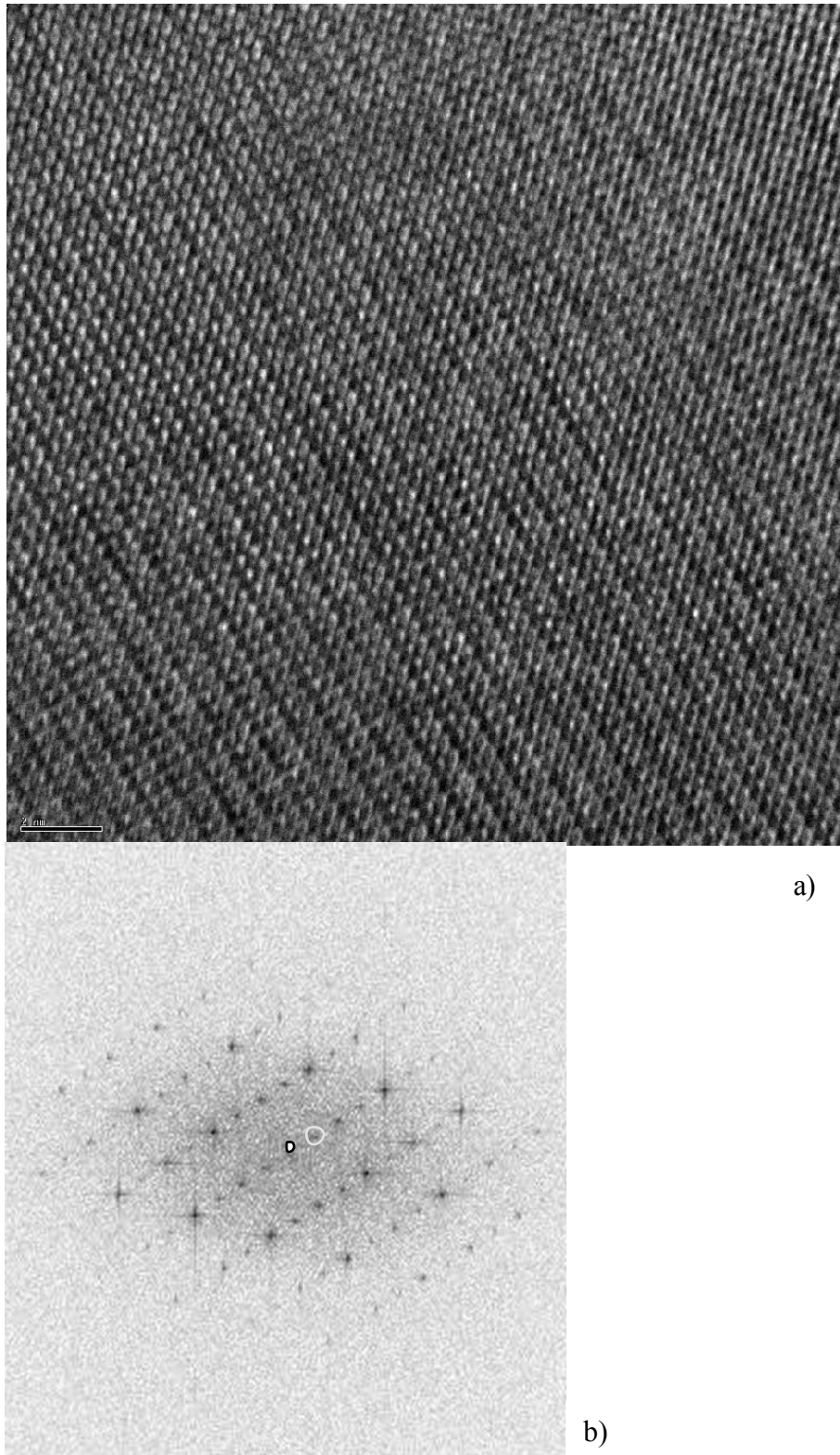
Fig 16 : Superlattice modulation, ordering along [100]
