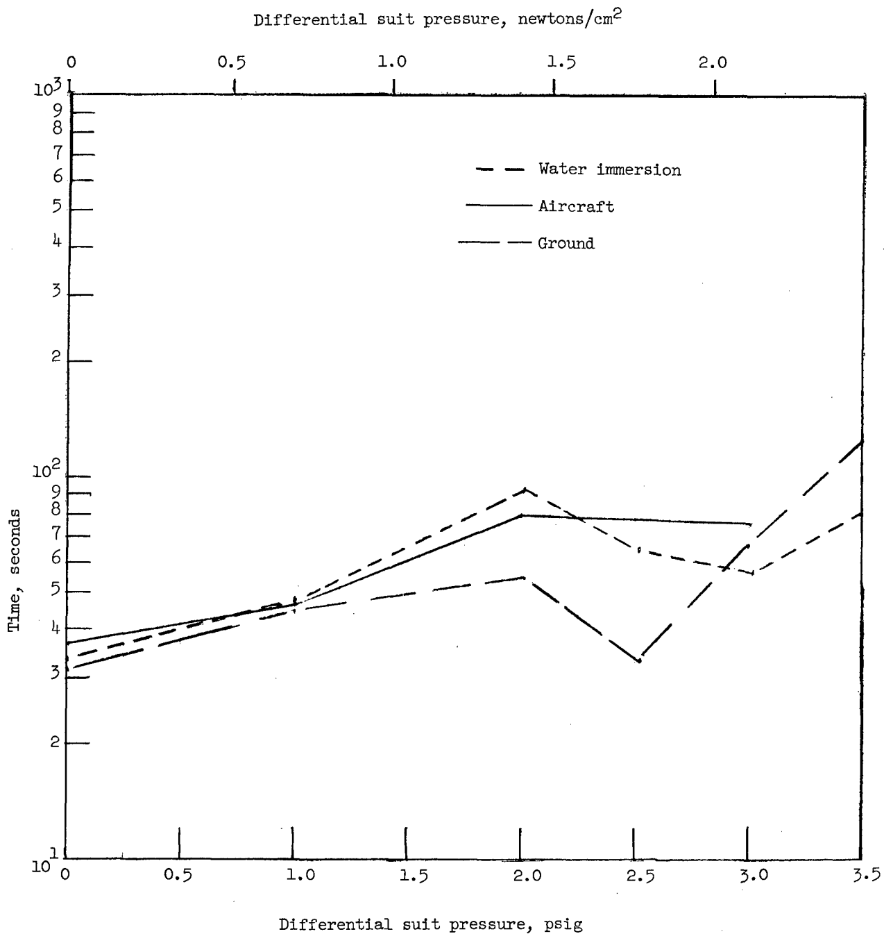
Figure 12.- Observed total ingress-egress times at various suit pressures for water-immersion, ground, and aircraft tests.
