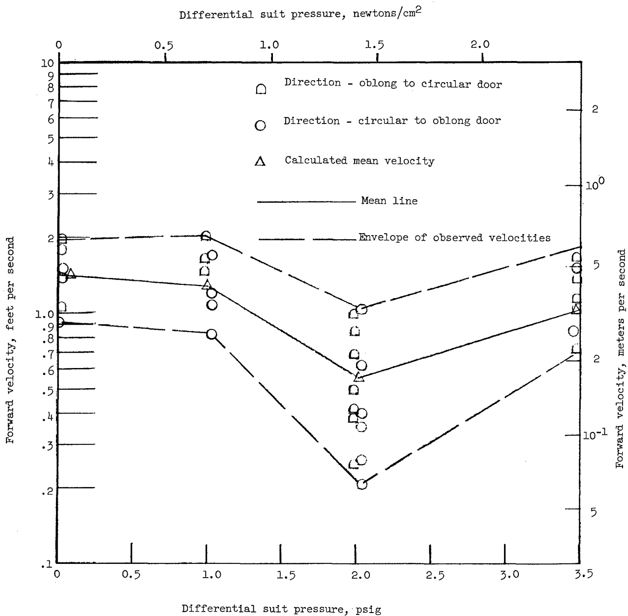
Figure 8.- Variation of observed forward velocity during ingress-egress maneuvers in water-immersion simulation with suit pressure.
