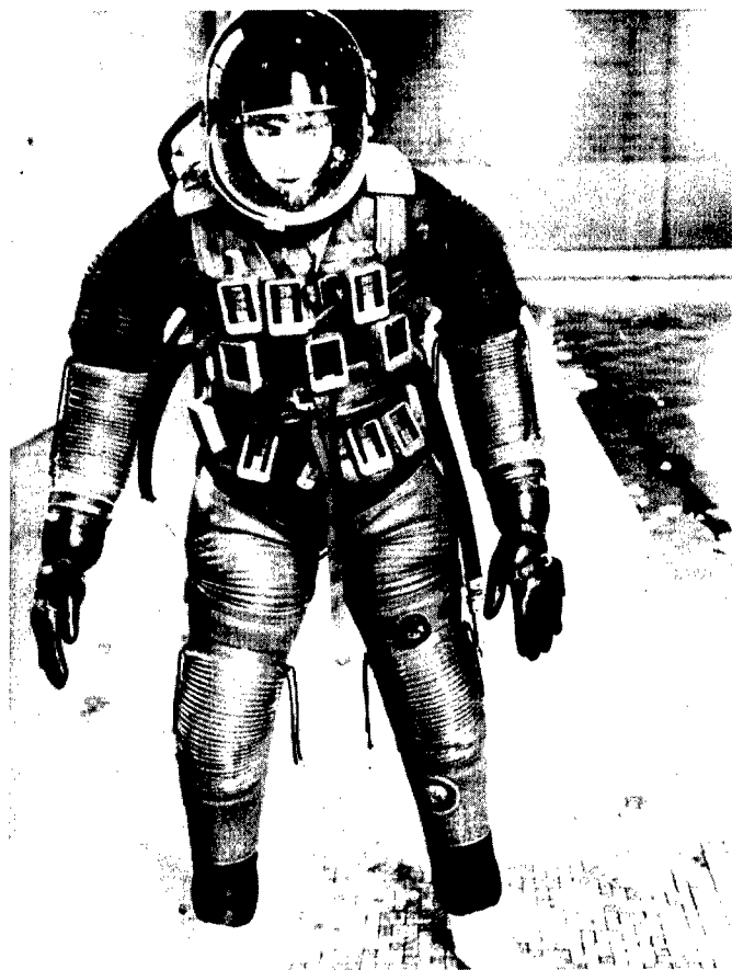
Figure 4.- Pressure-suited subject showing placement of external weights.
