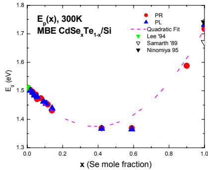
Fig. 4. CdSe x Te 1-x /Si bandgap as a function of Se composition ( 0 \leq x \leq 1 ) as determined by room temperature PL and PR measurements.
