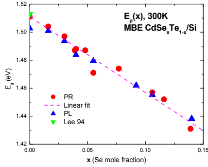
Fig. 3. CdSe x Te 1-x /Si bandgap as a function of Se composition ( x \leq 0.15 ) as determined by room temperature PL and PR measurements.
