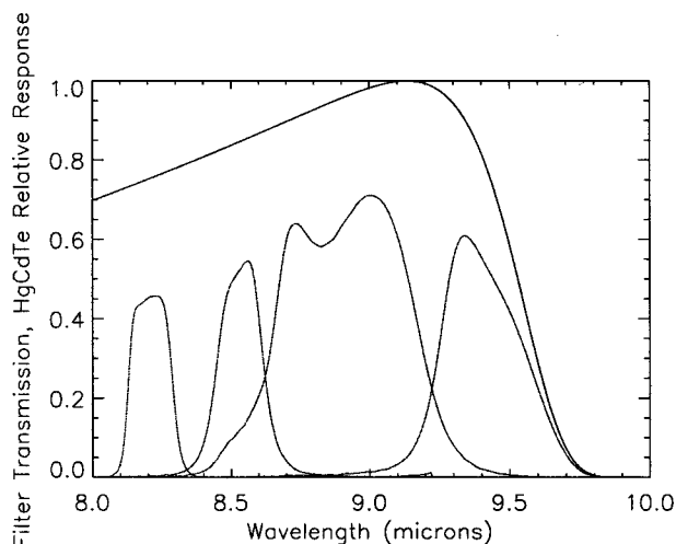
Fig. 2 Modeled spectral response of array and measured bandpass.
