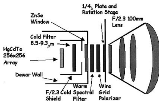
Fig. 1 Schematic of the LIP.
