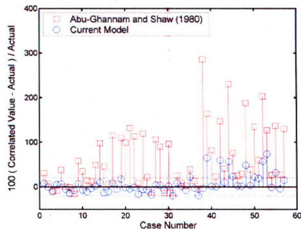
Figure 9. A comparison of the efficacy of the current transition-onset model for attached-flow with that of Abu-Ghannam and Shaw (1980).
