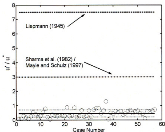
Figure 8. A comparison between the transition onset criteria of Liepmann (1945), Sharma et al. (1982), and Mayle and Schulz (1997) and the current attached-flow database.
