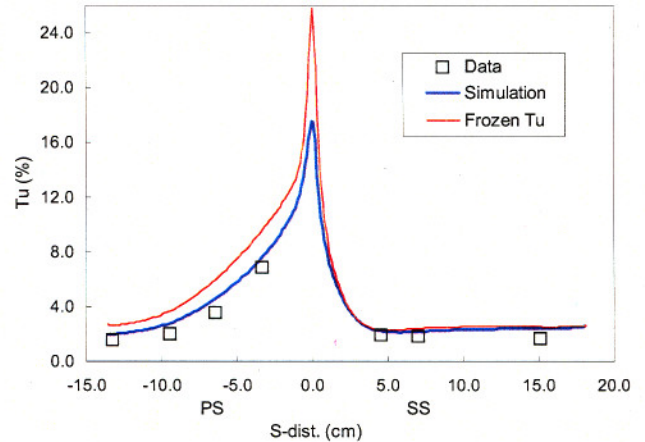
Figure 1. Measured and predicted distributions of freestream turbulence around the C3X airfoil. Data is from Ames (1994).
