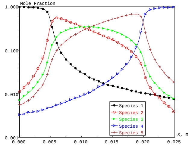
Figure 5: Distribution of the mole fraction of different species along the flow centerline for Kn_{II}=75
