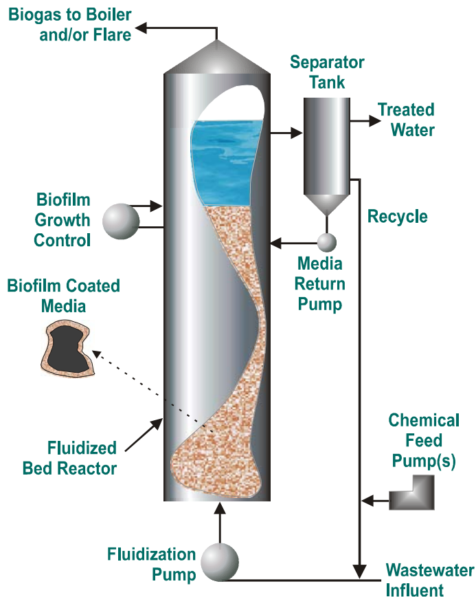
Figure 1. Conceptual drawing of an anaerobic granular activated carbon – fluidized bed reactor.
