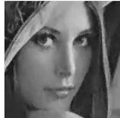
Quadtree scheme, cycle spinning with 16 shifts
