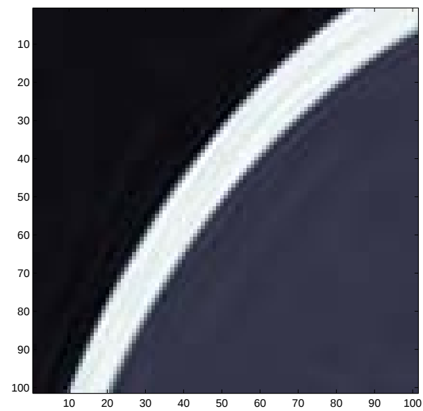
(f) Curvelets
