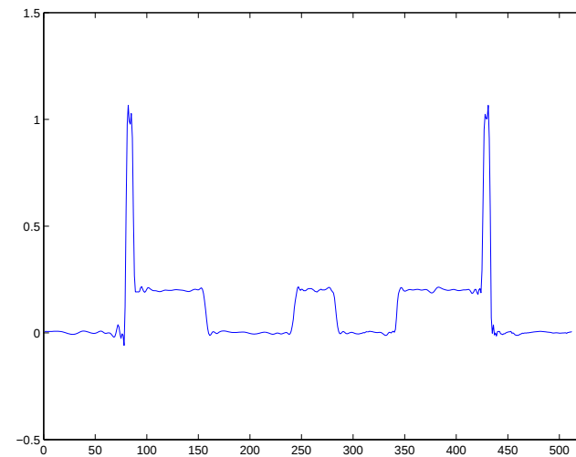
(b) Curvelets
