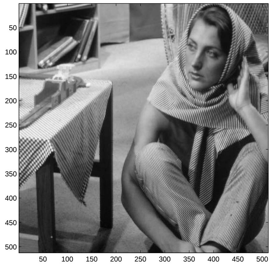
(p) Original
