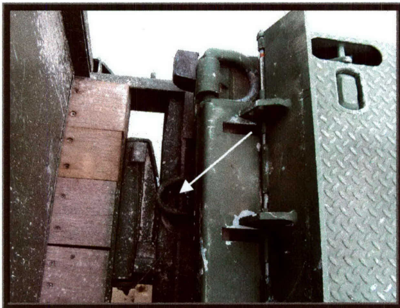
Photo 7. Interference of CROP with the Recessed Tiedowns
