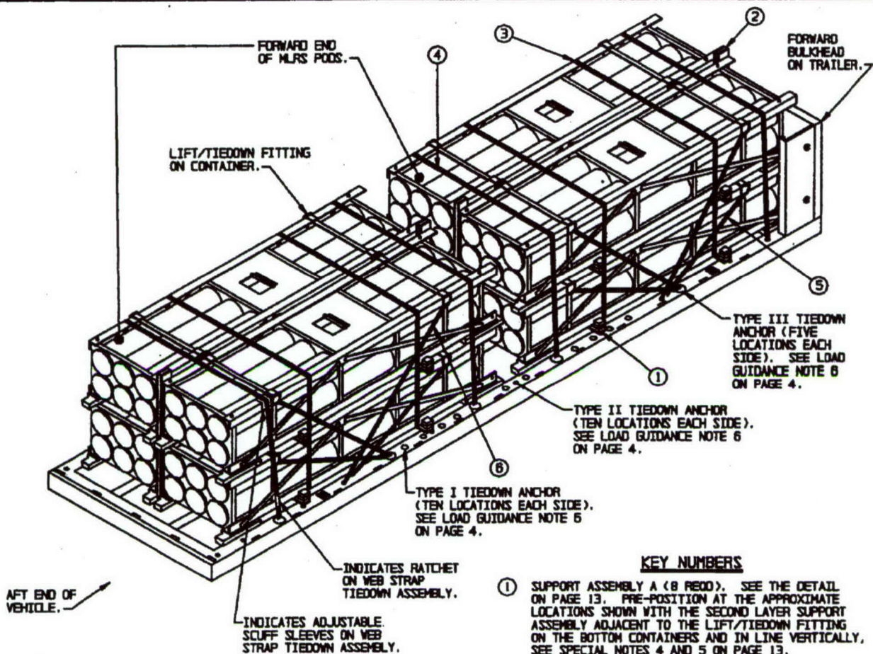
ISOMETRIC VIEW
