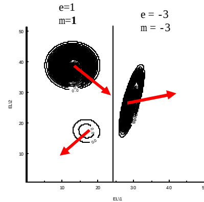
Fig. 1) A 20-fs pulse traverses a boundary that separates vacuum from a medium with \epsilon=-3 and \mu=-3 . The beam is seen to refract in an unusual direction, while the transmitted energy and momentum reorganize into a distorted wave front.
