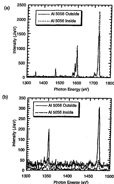
FIG. 1. (a) A comparison of the measured magnesium and aluminum H- and He-like emissions when Mg-bearing alloy (Al 5056) was placed in the outer (solid curve) or inner array (dotted curve) for a 40 mm diameter, 28 onto 14 wire nested implosions. (b) The same data with the range selected to highlight the Mg emissions.
