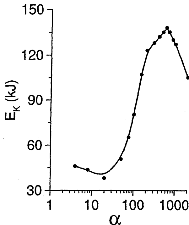
FIG. 8. The variation in the K-shell energy radiated in 200 ns as a function of the heat flux multiplier. The circuit resistance and \beta multiplier are the same as in Figs. 6 and 7. The calculated K-shell pulse had negligible amounts of emission following the main pulse. A spline fit is drawn to the calculated points.
