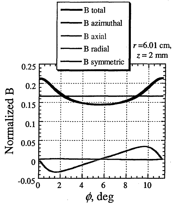
Figure 11. Magnetic field profiles for N_s = 32 , r = 6.01 cm, z = 2 mm.
