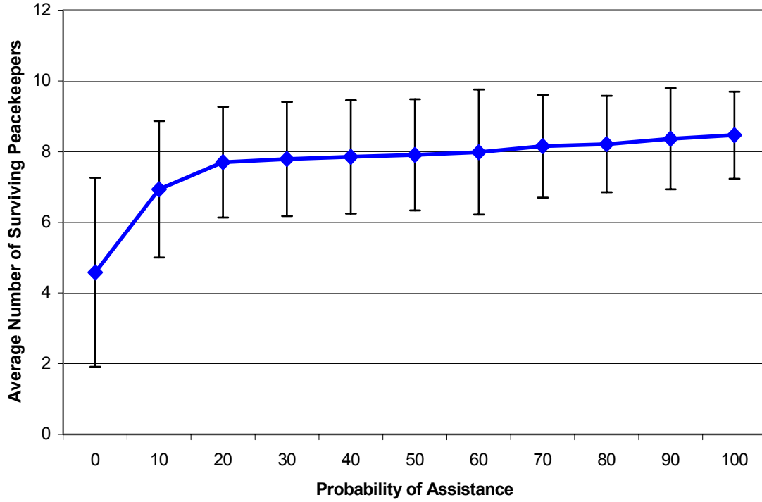
Figure 2: Plot of S_{avg} count against p_{scan}
