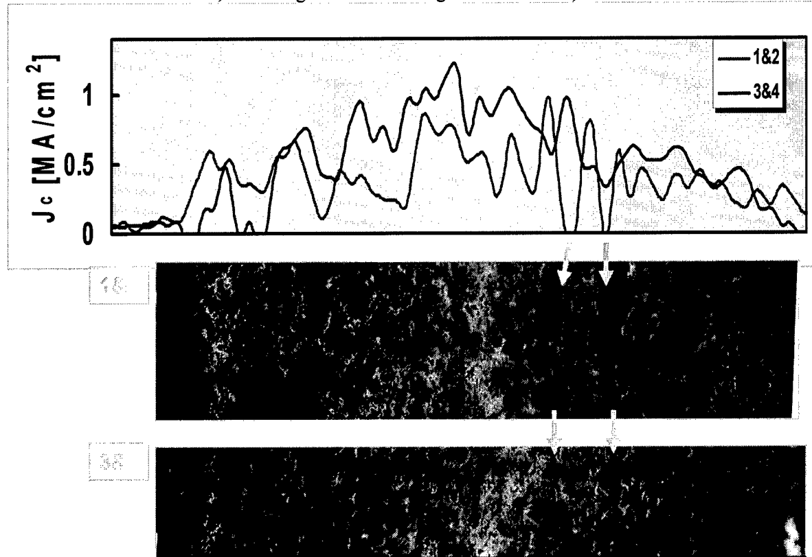
Figure 7. Magnetic knife profile of critical current density versus location, and corresponding MOI images. Both are taken after straining the YBCO coated conductor.
