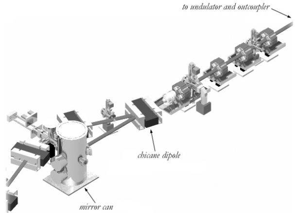
Figure 3.8: The source of useful THz radiation. Terahertz light is tapped from the chicane dipole just upstream of the undulator then transported up into the user facility.
