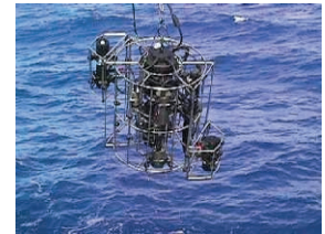
FIGURE 9. Submersible cage containing instruments used to measure ocean optical properties.
