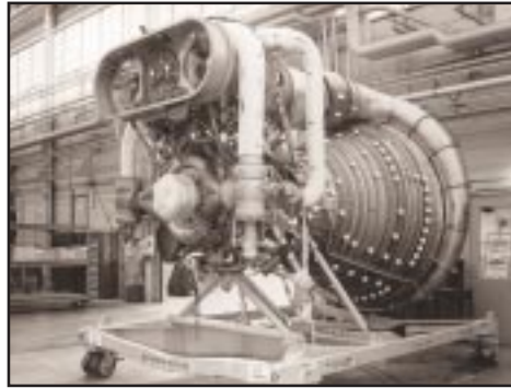
■ The F-1 engine.
