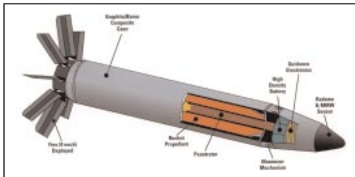
■ The X-Rod “smart” tank munition.
