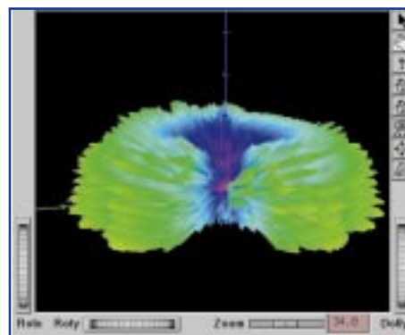
NEC-BSC volumetric pattern of the JTIDS antenna (AS-4400/URC) on the LHD-1 – stern view.
