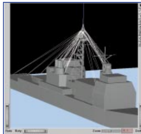
NEC-BSC ray visualization between relocated antennas 3-5 and 3-6 (AS-2810/SRCs) on the CG 47.
