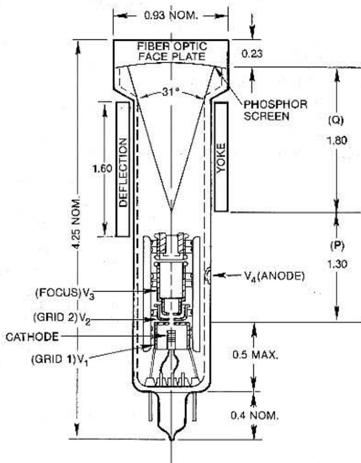
FIGURE 21 REPRESENTATIVE EMD/ESFL BIPOTENTIAL LENS MINIATURE CRT
