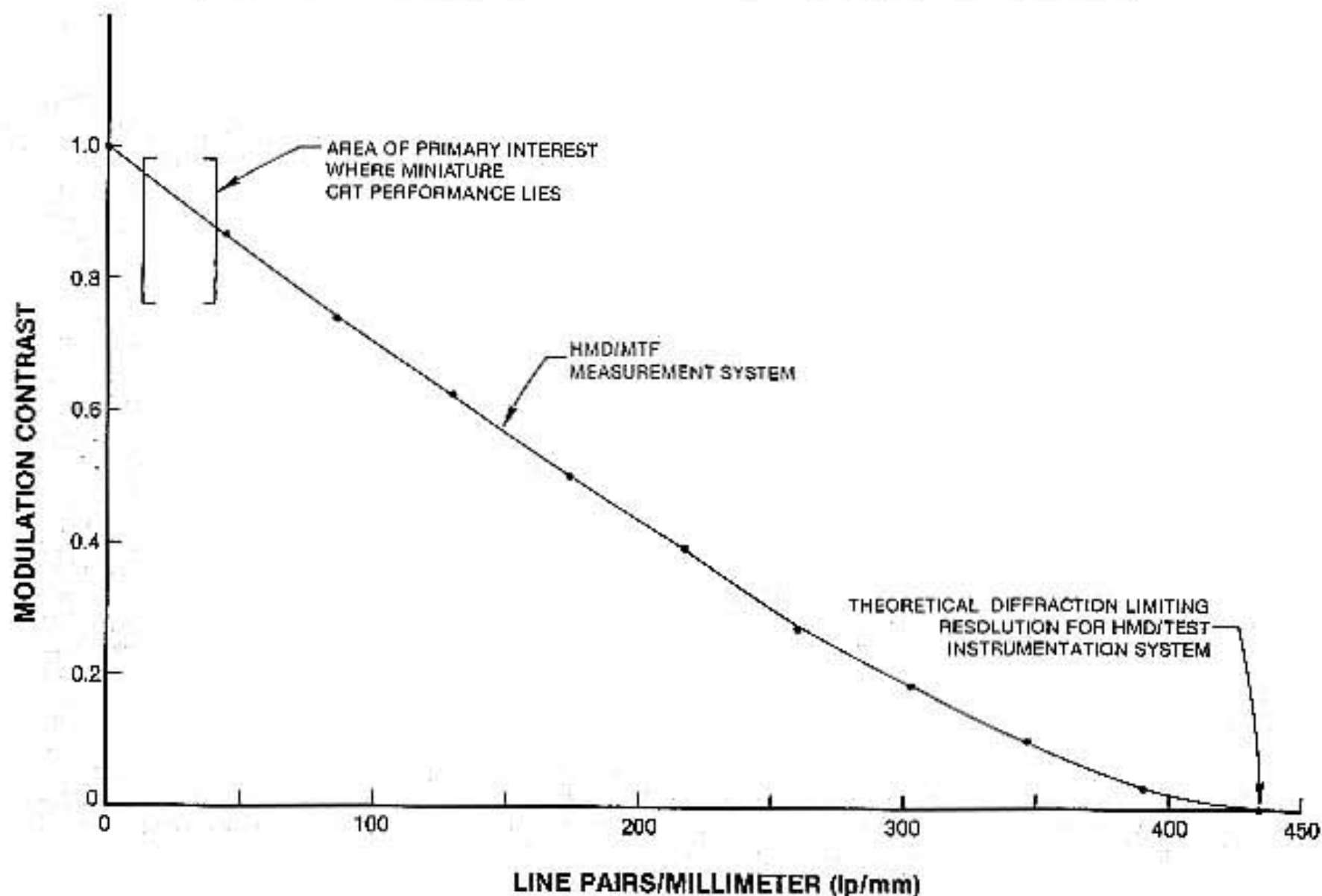
FIGURE 19 PLOT OF IDEALIZED OPTICAL MTF FOR MEASUREMENT SYSTEM/OPTICS
