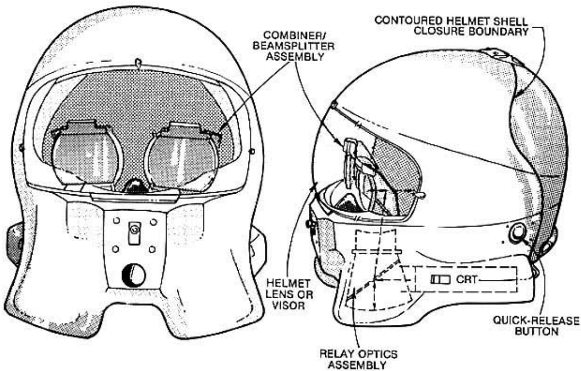
FIGURE 25 PROTOTYPE DUAL MIRROR OPTICS/HEADGEAR BREADBOARD
