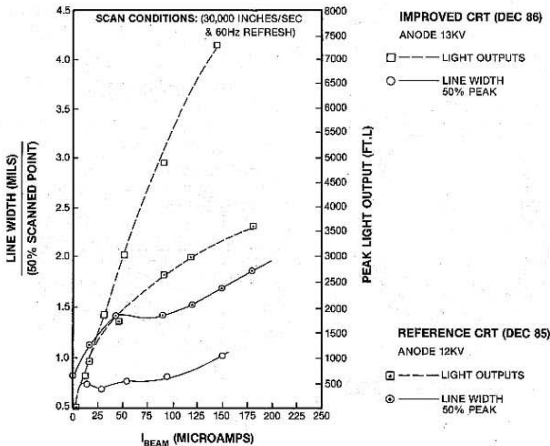
FIGURE 22 COMPARISON OF MINIATURE CRT PERFORMANCE IMPROVEMENTS
