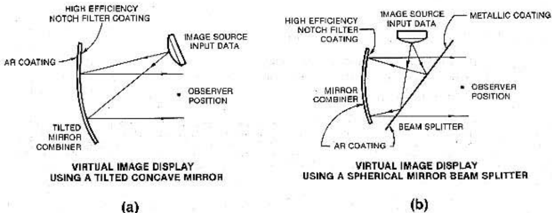
FIGURE 18 COMMON HMD COMBINER RELATIONSHIPS
