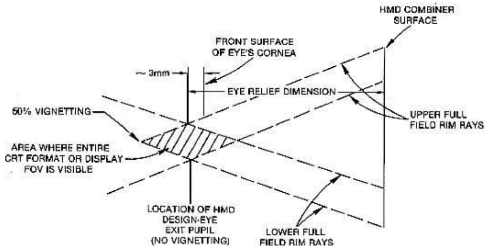
FIGURE 16 EXIT PUPIL/EYE RELATIONSHIPS
