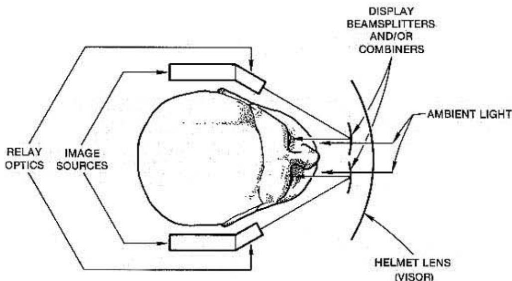
FIGURE 2 VPD HEAD/VISUAL SYSTEM RELATIONSHIPS
