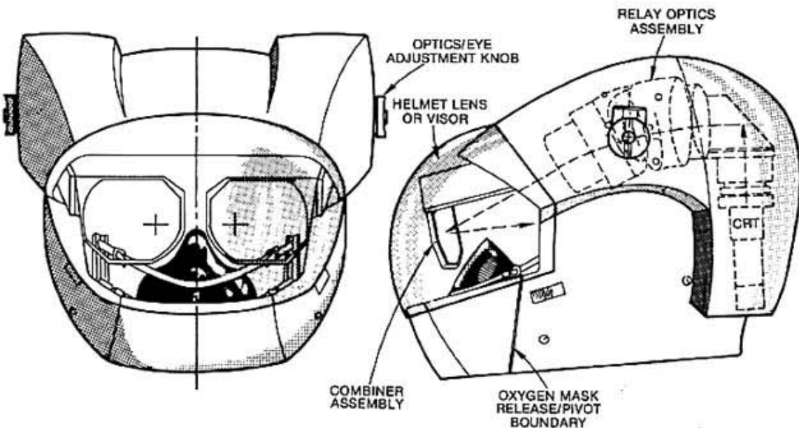
FIGURE 27 PROTOTYPE OFF-APERTURE OPTICS/HEADGEAR BREADBOARD
