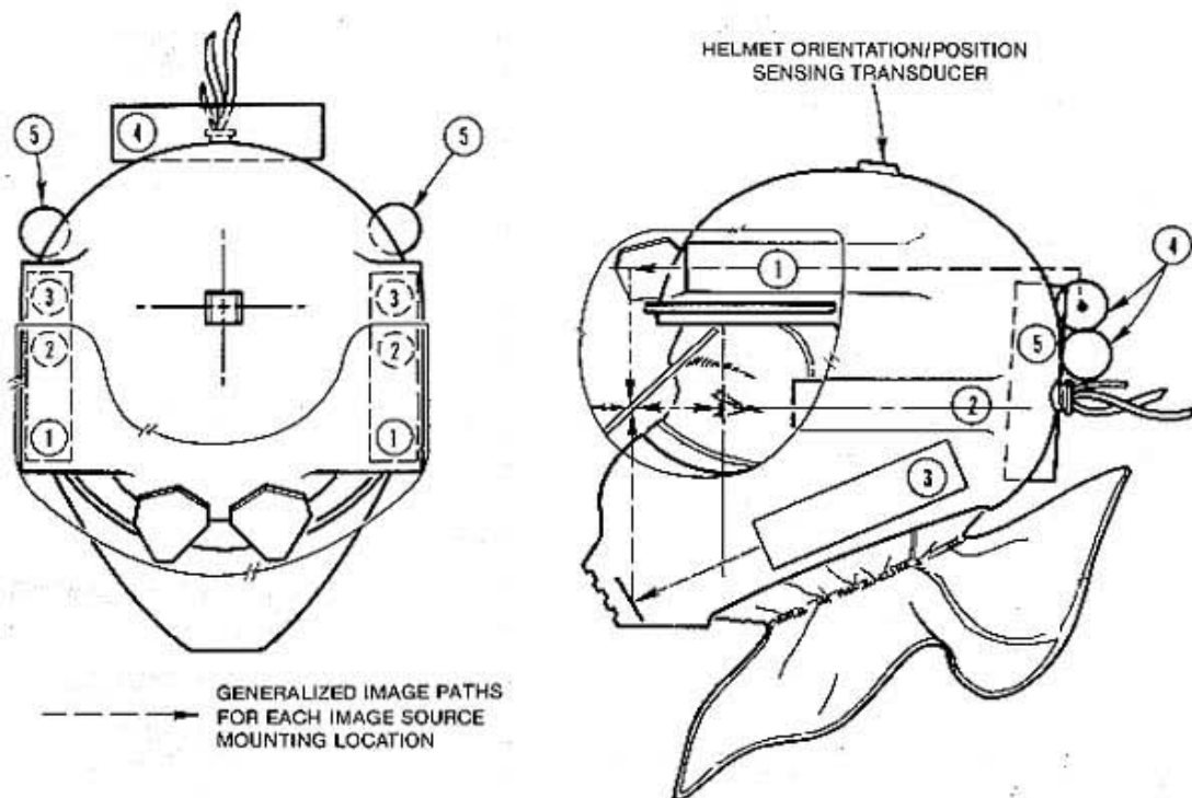
FIGURE 23 IES MOUNTING LOCATIONS FOR VPD HMD COMPONENTS
