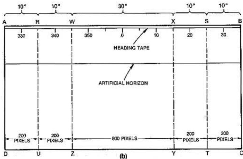
FIGURE 7 SCAN FORMAT RELATIONSHIPS FOR HYPOTHETICAL SENSOR/HMD COMBINATION
