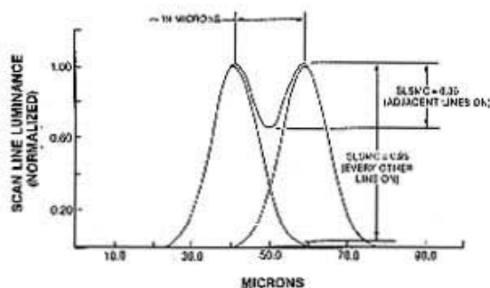
FIGURE 8 IMPACT OF MERGE POINT SELECTION FOR ADJACENT SCAN LINES
