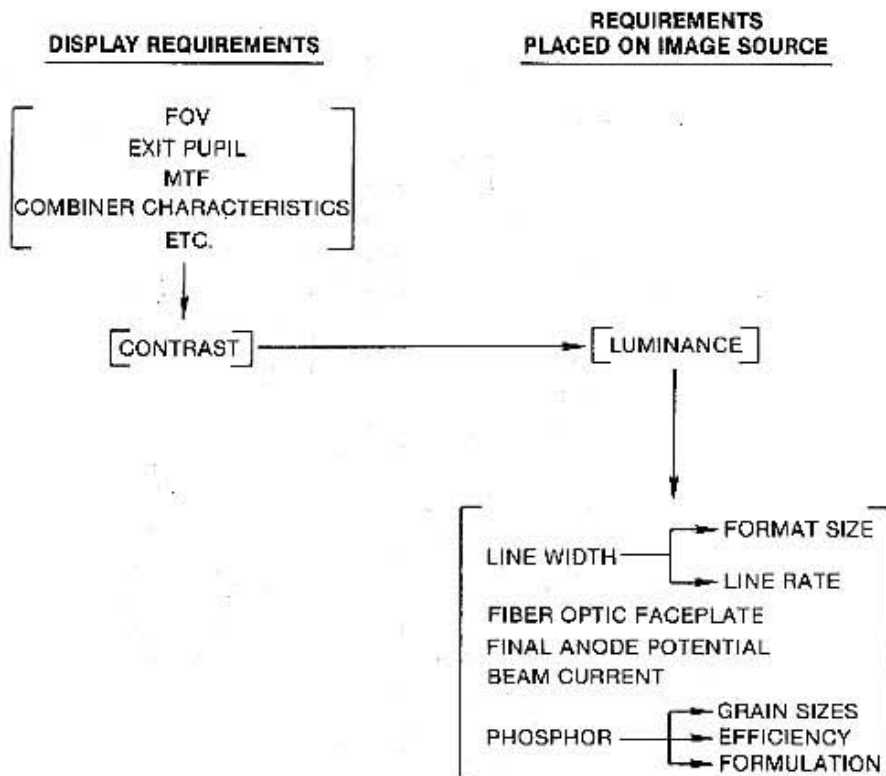
FIGURE 20 DISPLAY REQUIREMENT IMPACT ON IMAGE SOURCE PERFORMANCE
