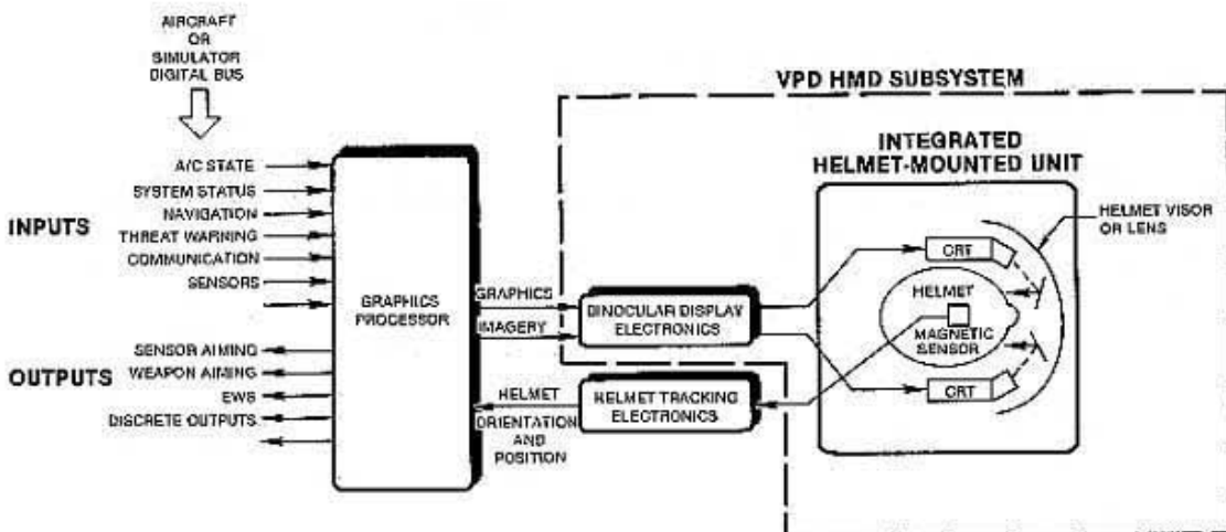
FIGURE 1 GENERIC VPD SYSTEM HARDWARE BLOCK DIAGRAM
