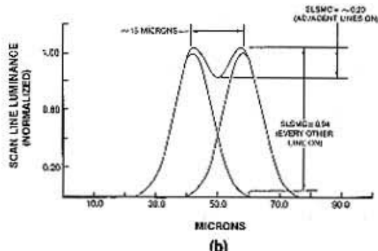
FIGURE 8 IMPACT OF MERGE POINT SELECTION FOR ADJACENT SCAN LINES
