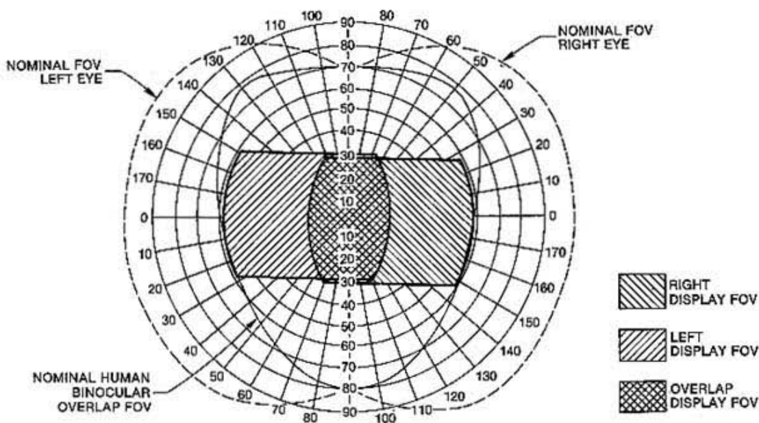
FIGURE 5 RELATIONSHIP OF HMD/EYE FOV
