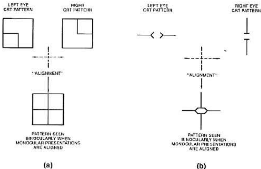
FIGURE 28 BINOCULAR DISPLAY ALIGNMENT PATTERNS
