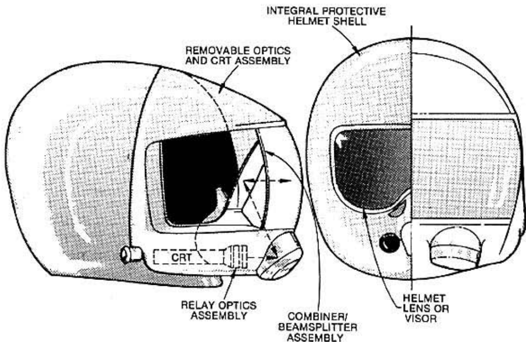
FIGURE 26 PROTOTYPE CATADIOPTRIC OPTICS/HEADGEAR BREADBOARD
