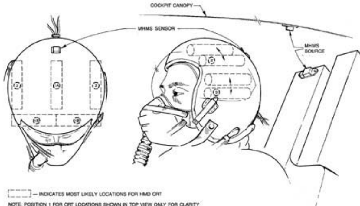
FIGURE 5 Normal Position Envelopes for Helmet-Mounted CRTs
