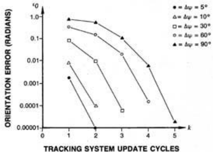
4a) Free Space Error Performance
