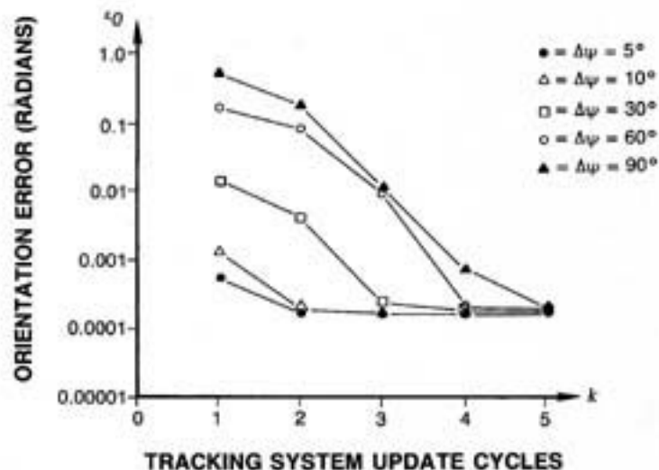
4b) Error Performance in the Presence of 2 Fixed Scatterers
