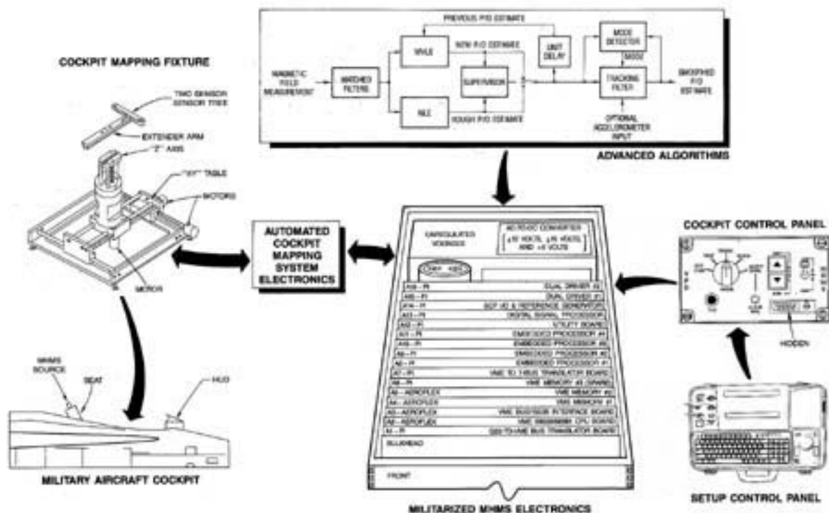
FIGURE 2 VPD MHMS System Concept
