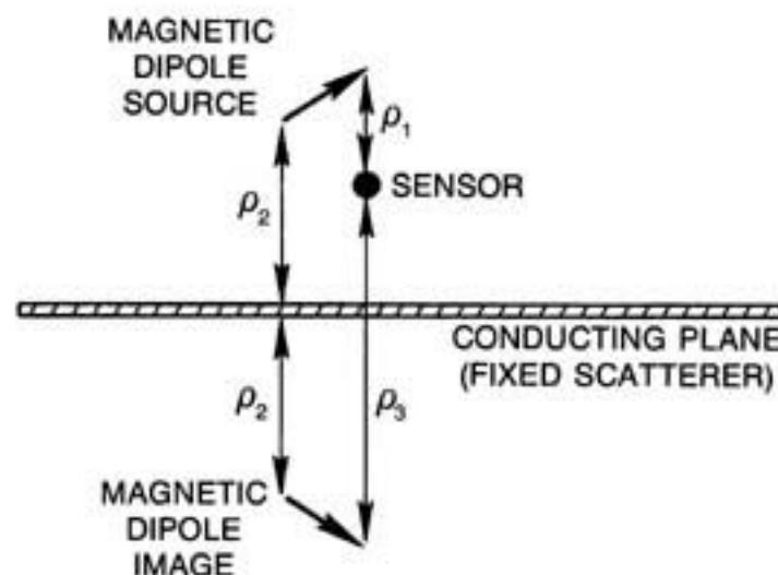
Figure 6 Fixed Scatterer Relationships
