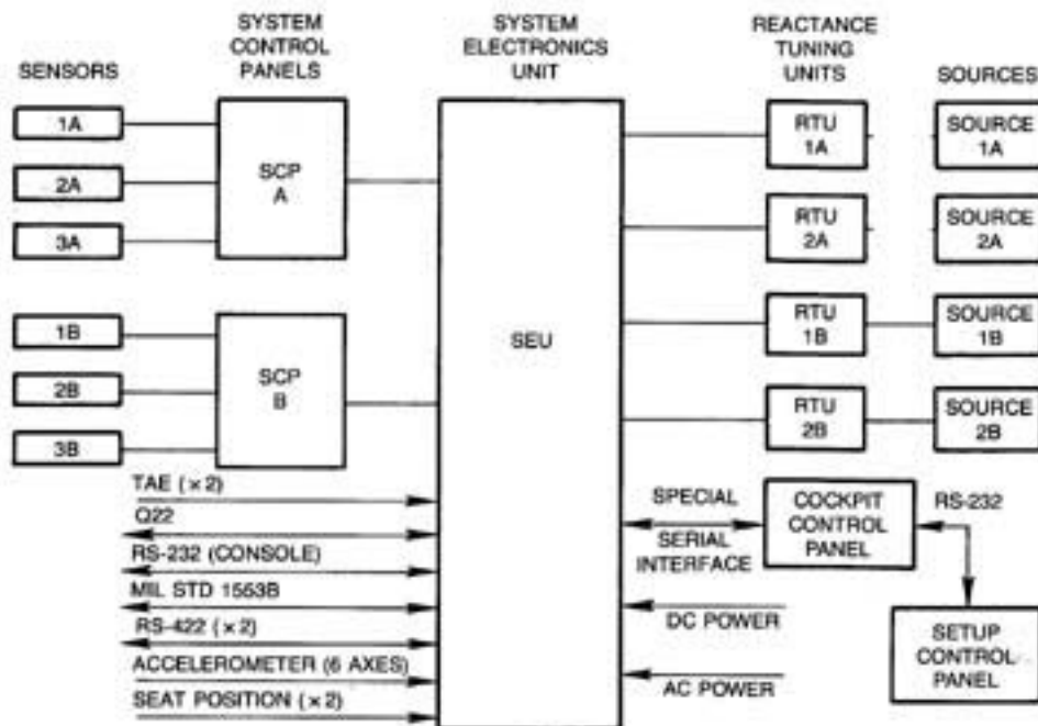
FIGURE 3 VPD MHMS Component Block Diagram
