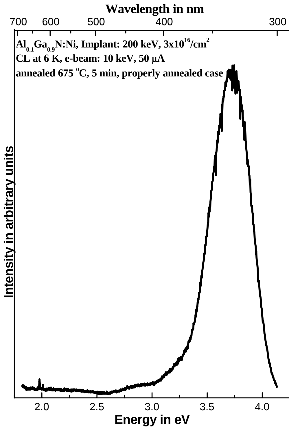
Figure 6. Cathodoluminescence spectrum of Al 0.1 Ga 0.9 N implanted with nickel and annealed for 5 minutes at 675 °C.
