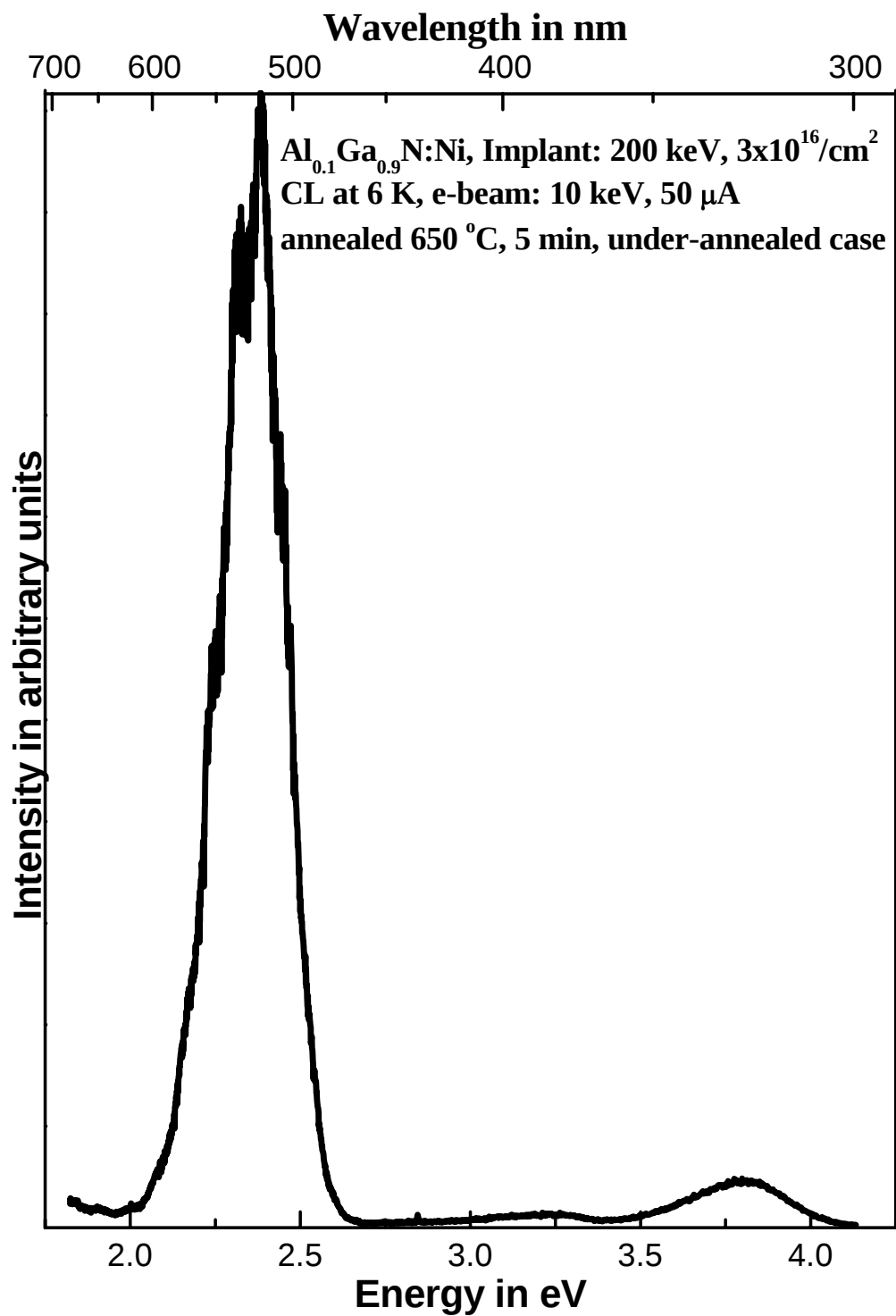
Figure 5. Cathodoluminescence spectrum of \text{Al}_{0.1}\text{Ga}_{0.9}\text{N} implanted with nickel and annealed for 5 minutes at 650\text{ }^\circ\text{C} .
