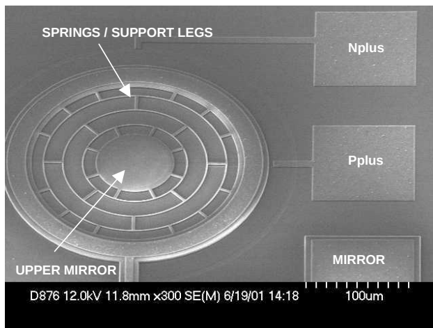
Figure 1. Entire MEMS USA sensor including the three contacts.
