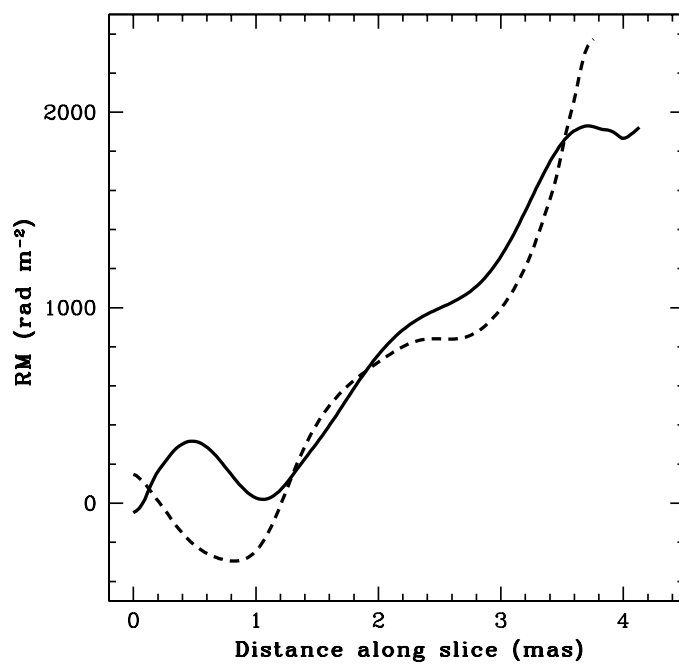
Fig. 3.— Rotation Measure image slices perpendicular to the jet axis for both epoch 2000.07 (dashed) and 2000.61 (solid). The region of the slice is indicated by the solid line in Fig. 1.
