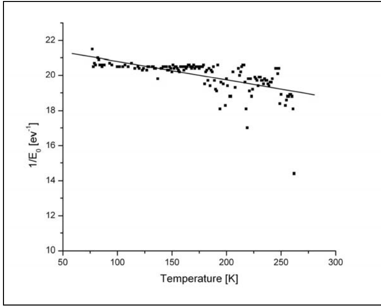
Figure 107. Reciprocal tunneling parameter, E_0 .
