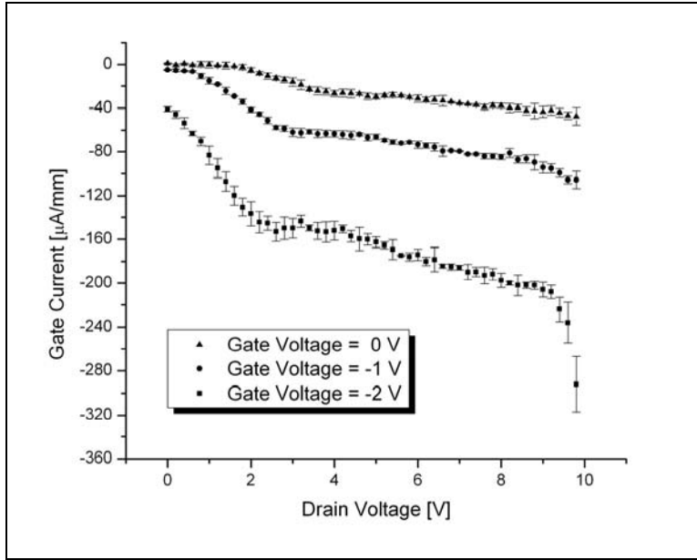
Figure 74. A29: Pre-irradiation gate leakage characteristics.
