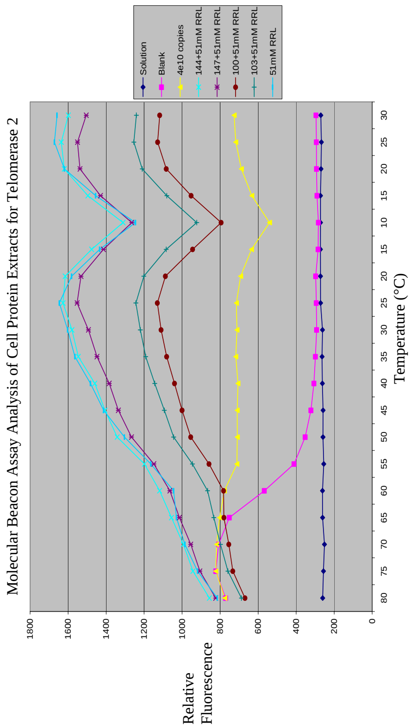
Figure 31. Molecular Beacon Assay Analysis of Cell Protein Extracts for Telomerase 2 The solution sample represented the background readings for FAM by the ABI prism. The blank solution represented the molecular beacon's natural thermodynamic stability through the temperature range. The 4e10 oligo copies/ \mu L showed the molecular beacon's thermodynamic nature through the temperature range in the presence of target entity. The experimental samples demonstrated an increase in fluorescence beginning with the telomerase negative samples (100 + 51mM RRL, 103 + 51mM RRL) progressing to the 51mM RRL sample and the telomerase positive samples (147 + 51mM RRL, 144 + 51mM RRL).
