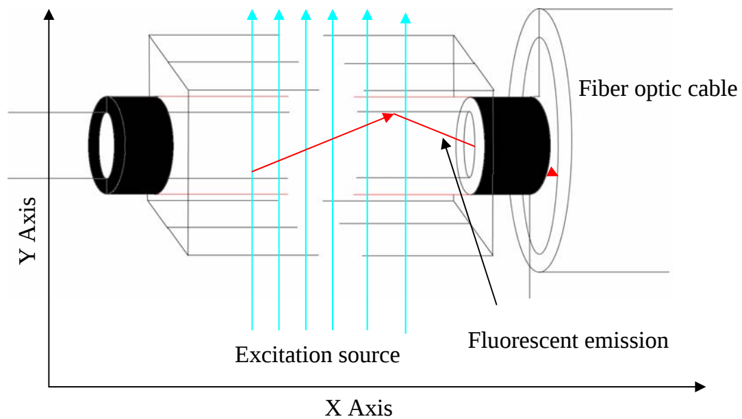
Figure 7. Illustration of Transverse Excitation/ Axial Detection This picture illustrates the LCWG placement in the PDMS chip and the cushion of air that would surround the LCWG. The excitation source would emit from the Y axis and the fluorescent emission for the MB would be detected on the X axis.
