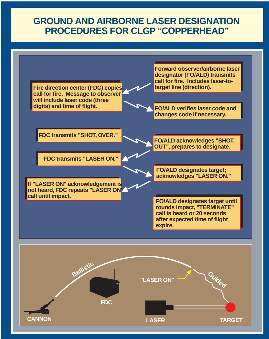
Figure B-A-1. Ground and Airborne Laser Designation Procedures for CLGP "COPPERHEAD"
