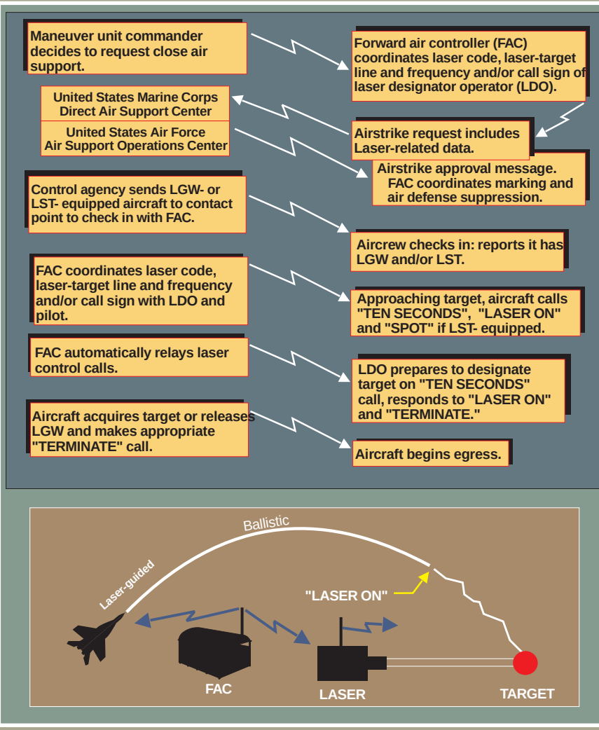
Figure B-B-1. Procedures for Aircraft With Laser-Guided Weapons and Laser Spot Trackers
