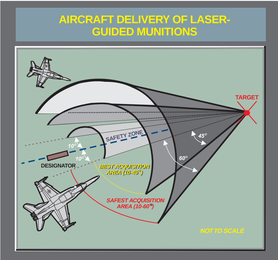
Figure III-1. Aircraft Delivery of Laser-Guided Munitions
