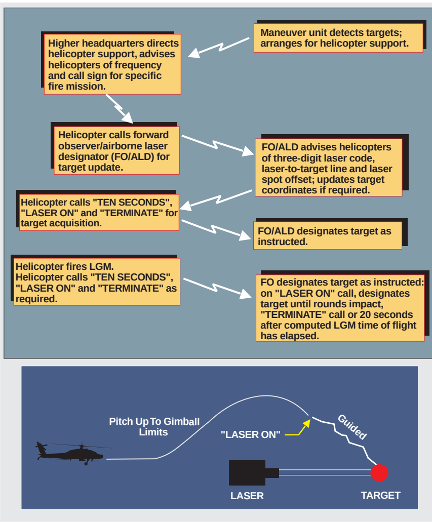
Figure B-C-1. Procedures for Helicopters With Laser-Guided Missiles and Remote Designator
