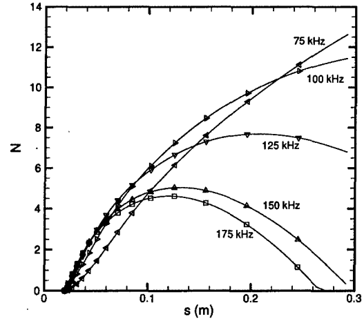
Figure 14: Maximum N factors obtained from many combinations of frequency, spanwise wavenumber, and starting location for the sharp cone at Mach 3.5.
