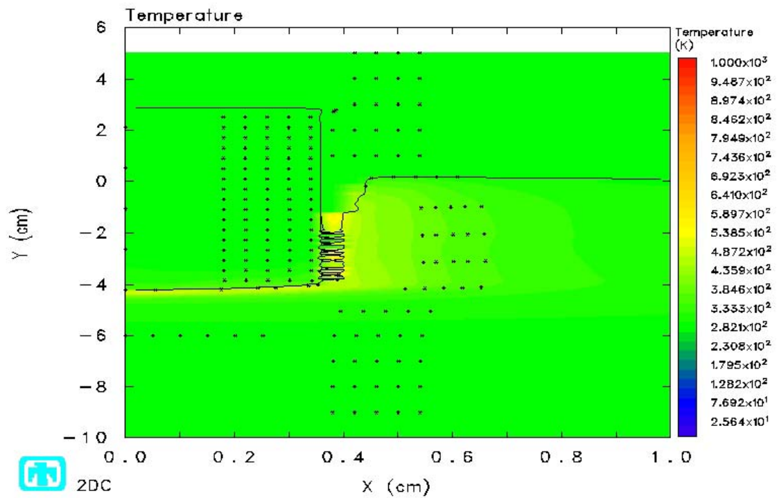
Figure 4.8 Temperature at 50 \mu\text{s} , Boundary Layer, \mu = 0.06
