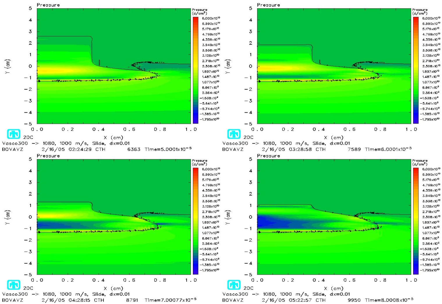
Figure 4.23 Pressure Contours at 50, 60, 70, and 80 \mu s, Slide Line
