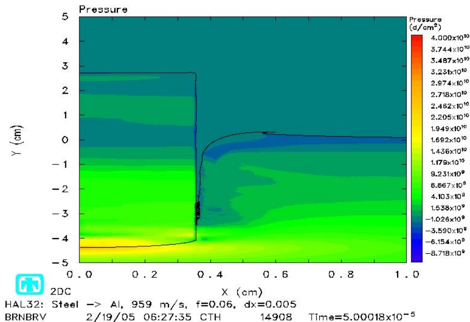
Figure 4.19 Pressure at 50 \mu s, .005cm Mesh, Boundary Layer
