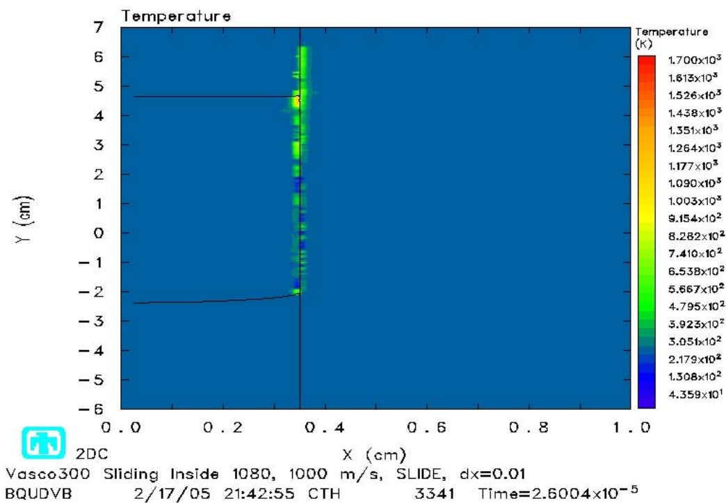
Figure 4.40 Temperature at 26 \mu\text{s} , Slide Line
