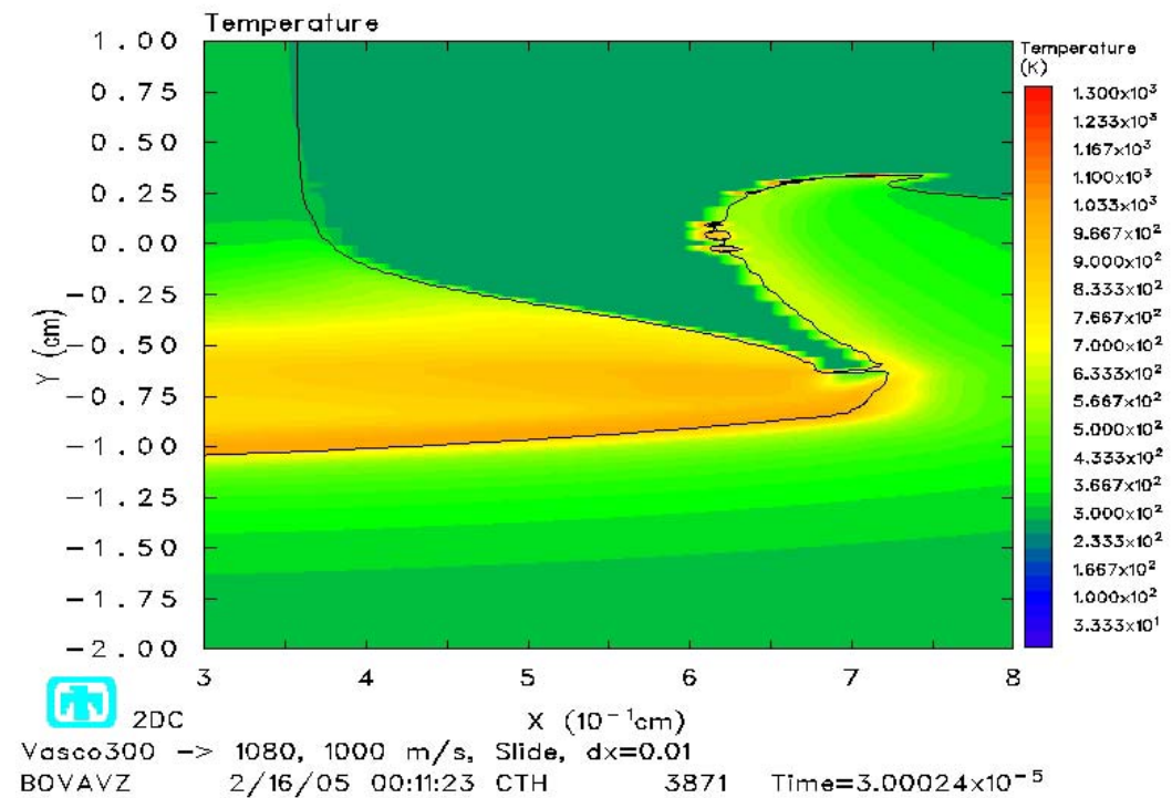
Figure 4.27 Temperature at 30 \mu s, Slide Line
