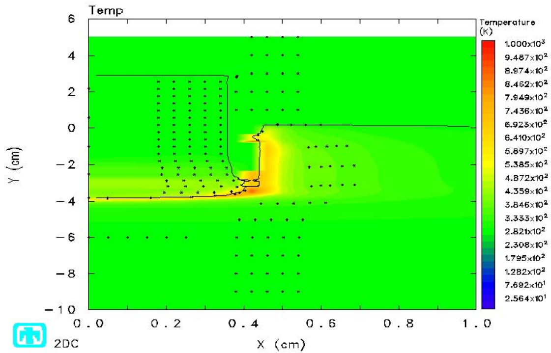
Figure 4.7 Temperature at 50 \mu\text{s} , Slide Line
