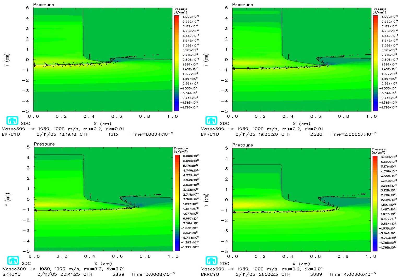
Figure 4.24 Pressure Contours at 10, 20, 30, and 40 \mu s, Boundary Layer
