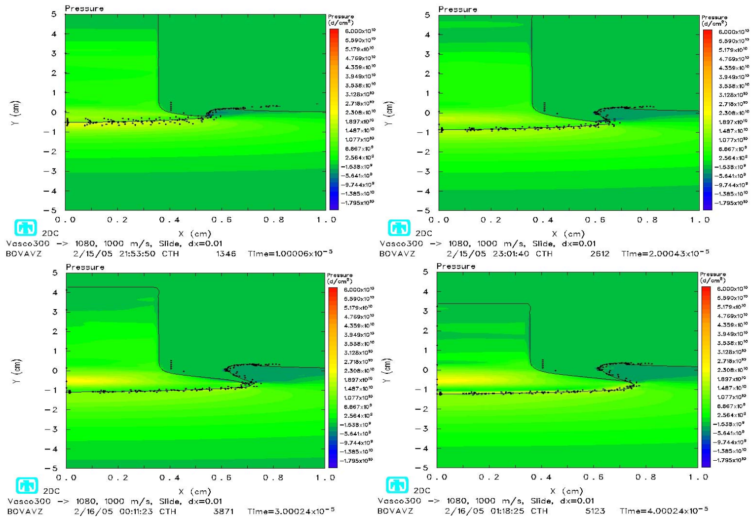
Figure 4.22 Pressure Contours at 10, 20, 30, and 40 \mu\text{s} , Slide Line
