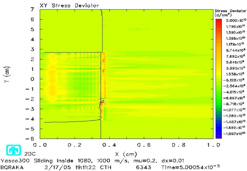
Figure 4.42b Deviatoric Shear Stress at 50 \mu\text{s} , BOUNDARY LAYER
