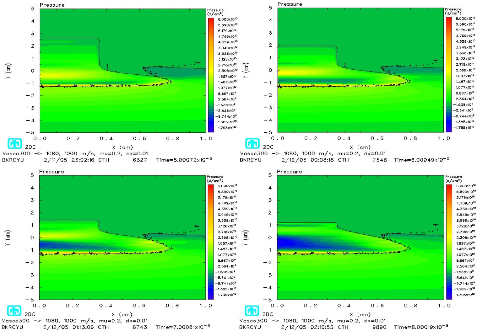
Figure 4.25 Pressure Contours at 50, 60, 70, and 80 \mu s, Boundary Layer
