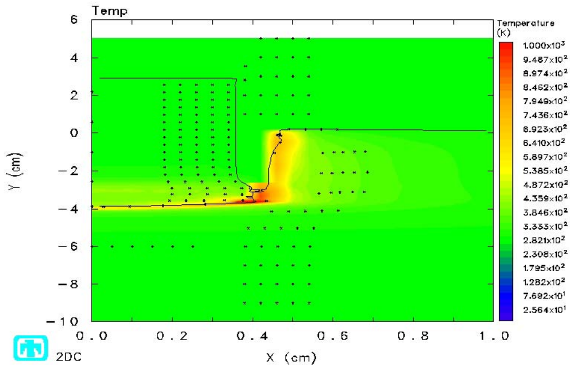
Figure 4.6 Temperature at 50 μs, No Slide Line
