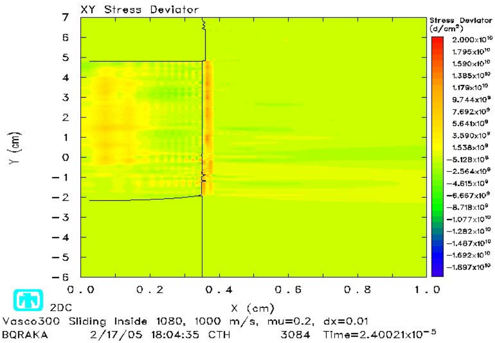
Figure 4.42a Deviatoric Shear Stress at 24 \mu\text{s} , BOUNDARY LAYER
