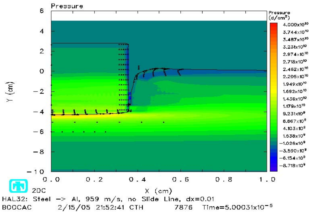
Figure 4.10 Pressure Contour at 50 \mu s, No Slide Line
