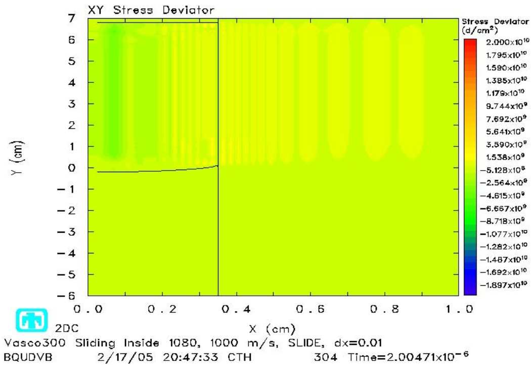
Figure 4.39 Deviatoric Shear Stress at 2 \mu\text{s} , Slide Line
