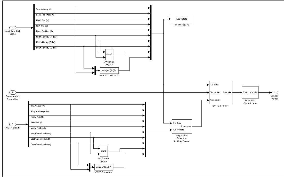
Figure 38. Final Controller Simulink® Model
