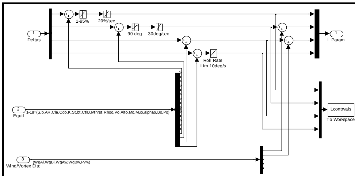
Figure 104. L Param w/ Limits Block
